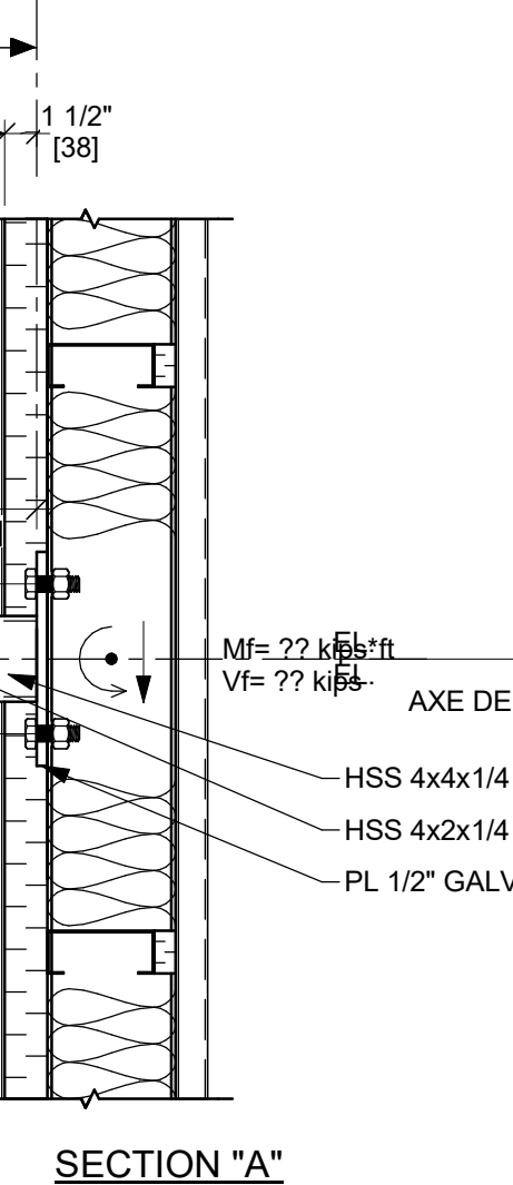
SECTION "A"
