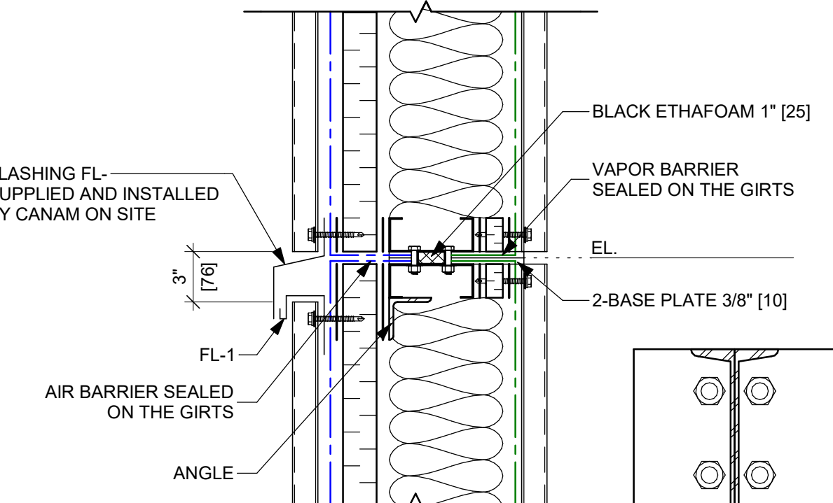
Murox stacked panels CI R-25 & CI R-27
