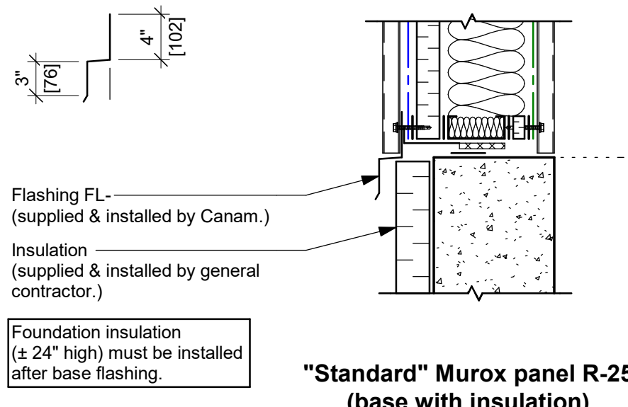
"Standard" Murox panel R-25 (base with insulation)
