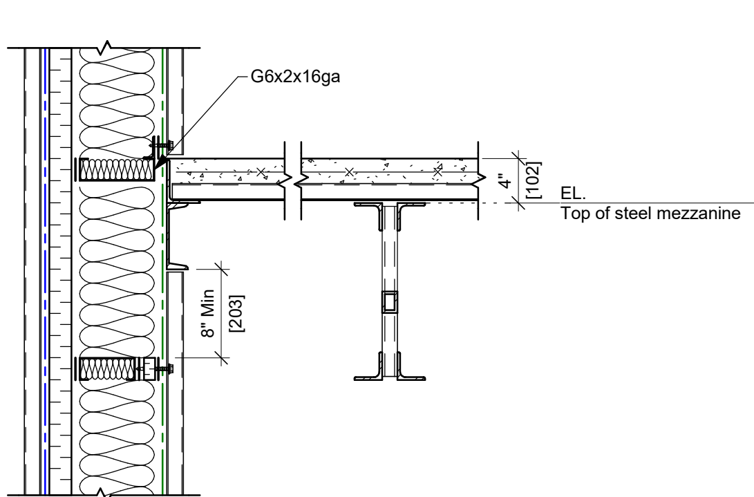
Panel at the mezz R-25 & R-27 (C6) (siding, liner, joist para.)
