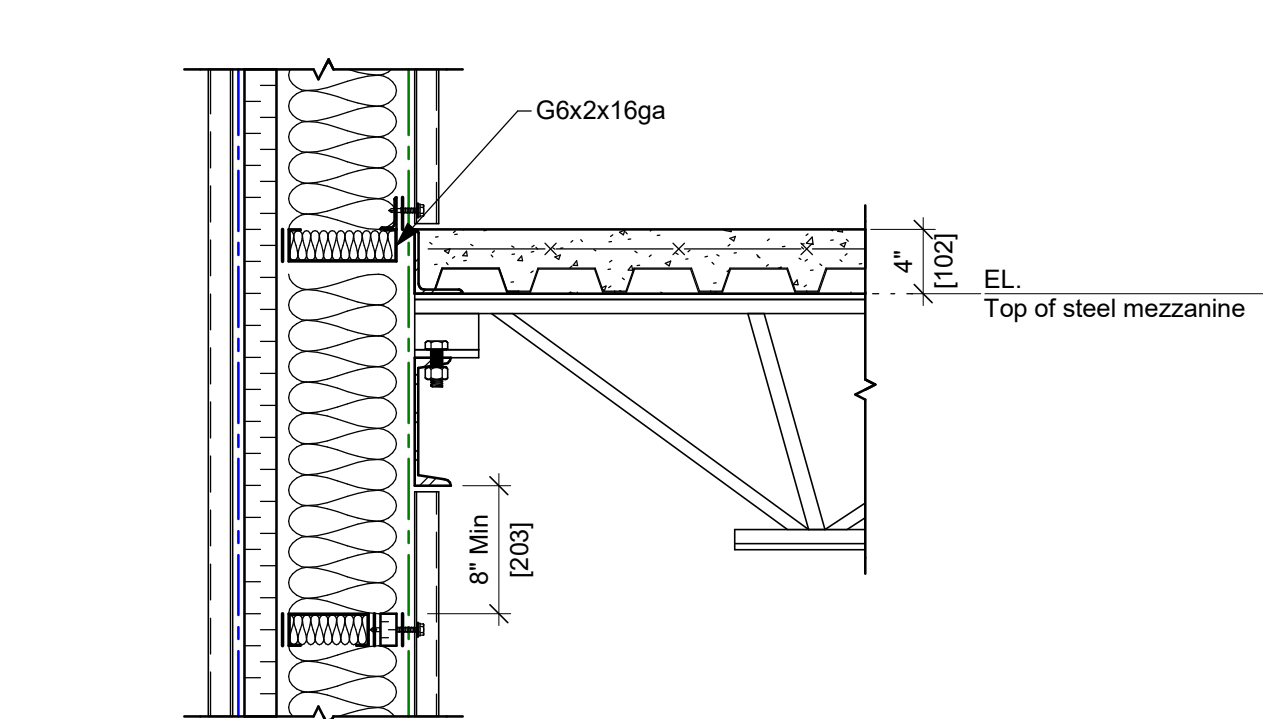
Panel at the mezz R-25 & R-27 (C6) (siding, liner, joist perp.)
