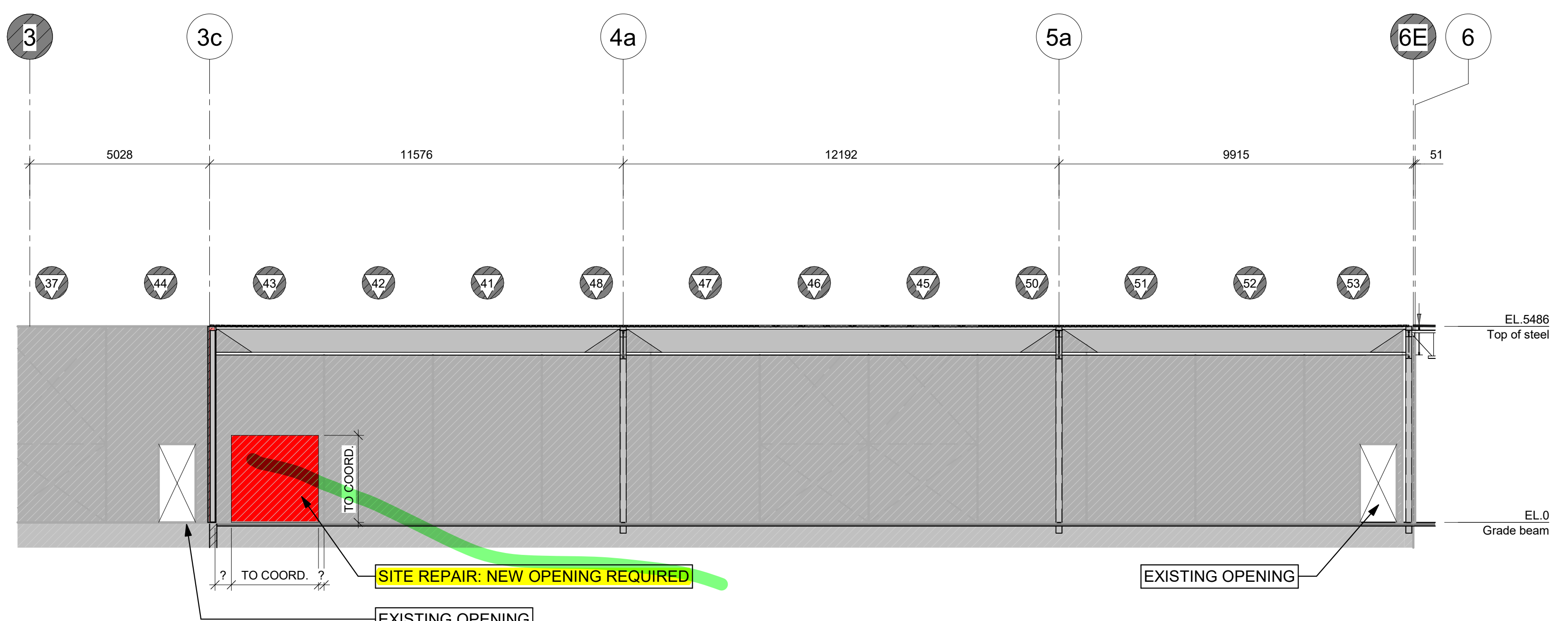
ELEVATION LINE F - EXISTING PANELS 1:100
