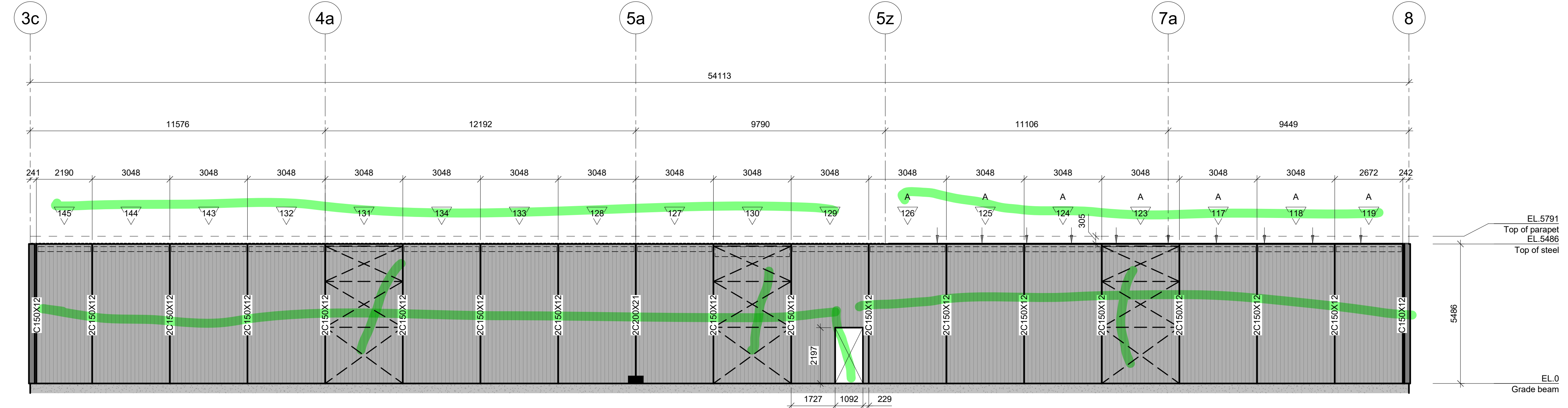
ELEVATION LINE H 1:100 NON LOAD BEARING PANELS BRACING ROD 1"ø TYP UNO
