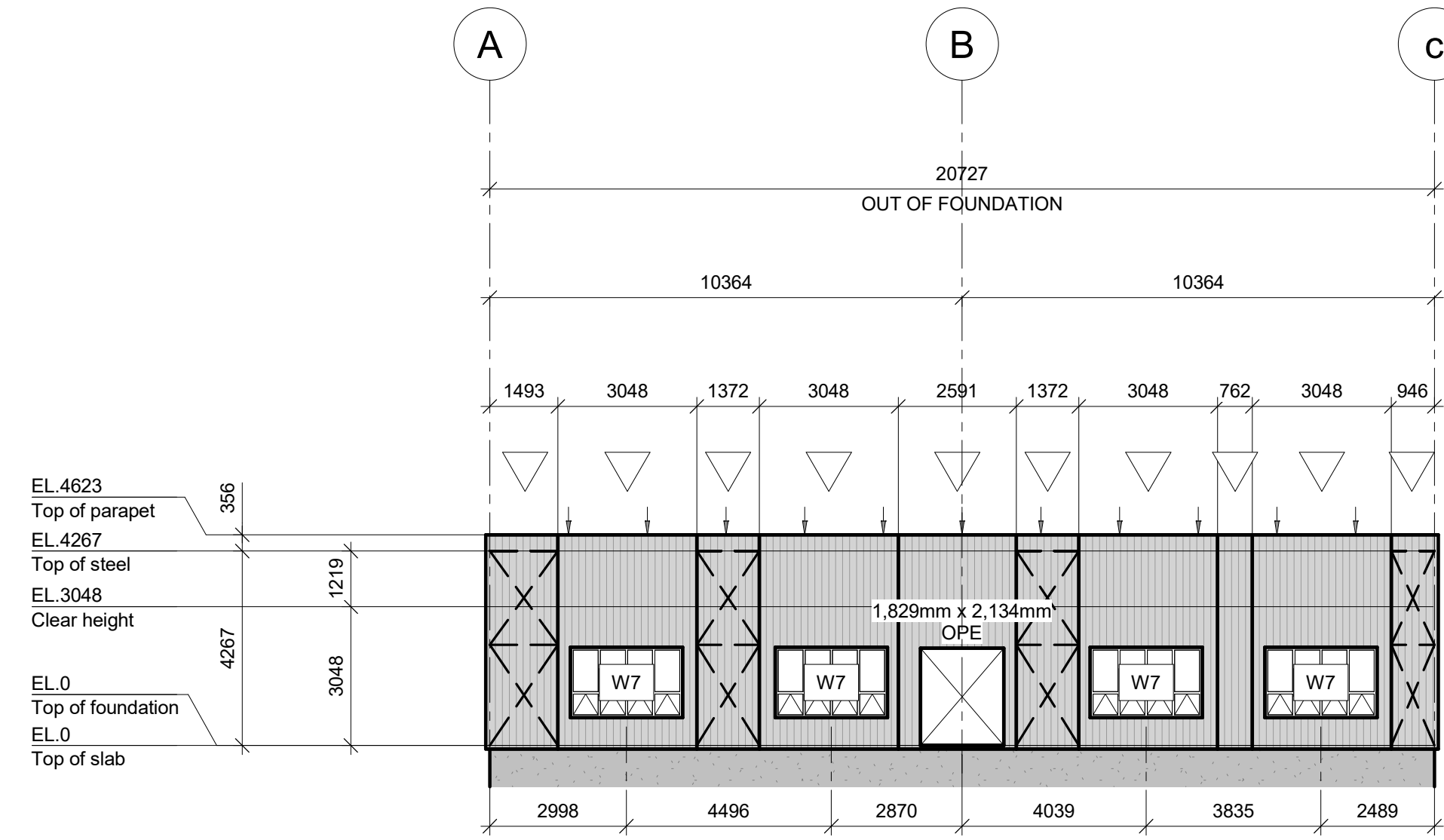
ELEVATION LINE 5 (EAST) 1 : 125
