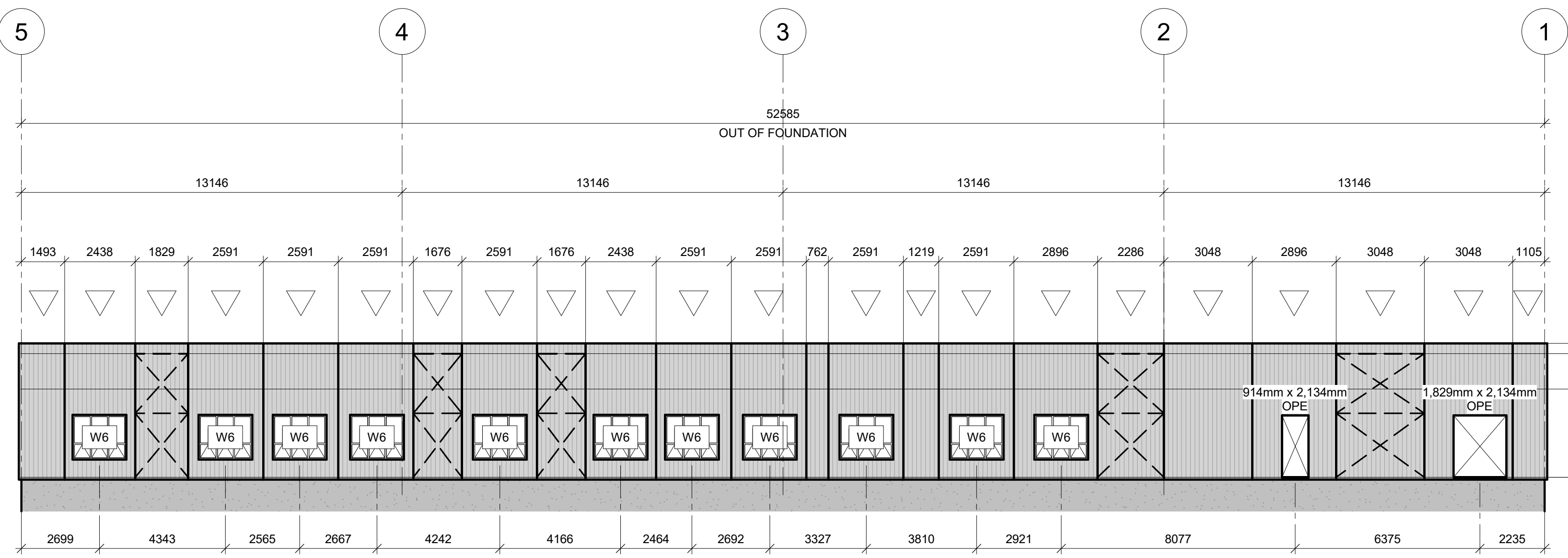
ELEVATION LINE C (NORTH) 1 : 125
