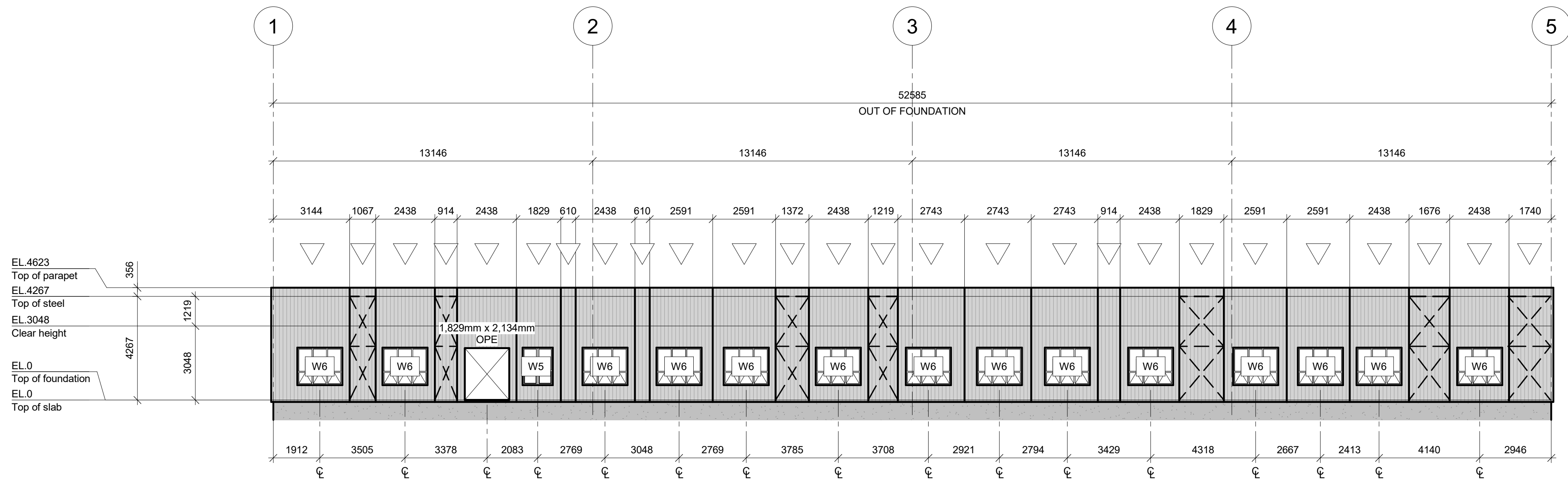
ELEVATION LINE A (SOUTH) 1 : 125
