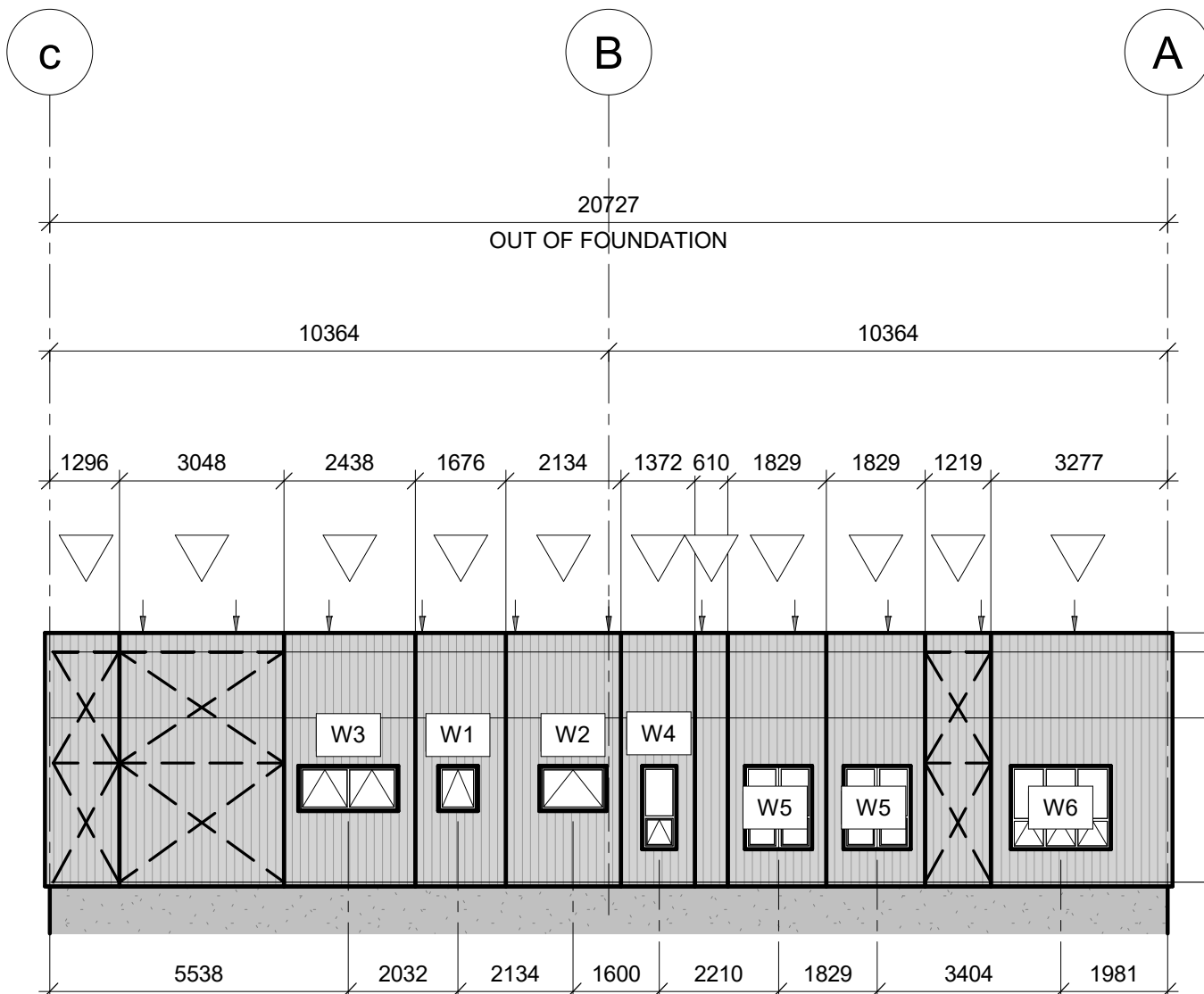
ELEVATION LINE 1 (WEST) 1 : 125
