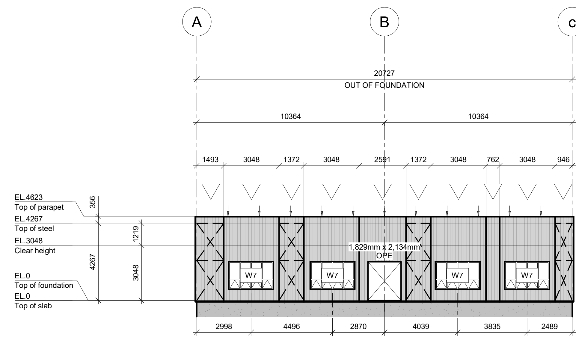
ELEVATION LINE 5 (EAST) 1 : 125
