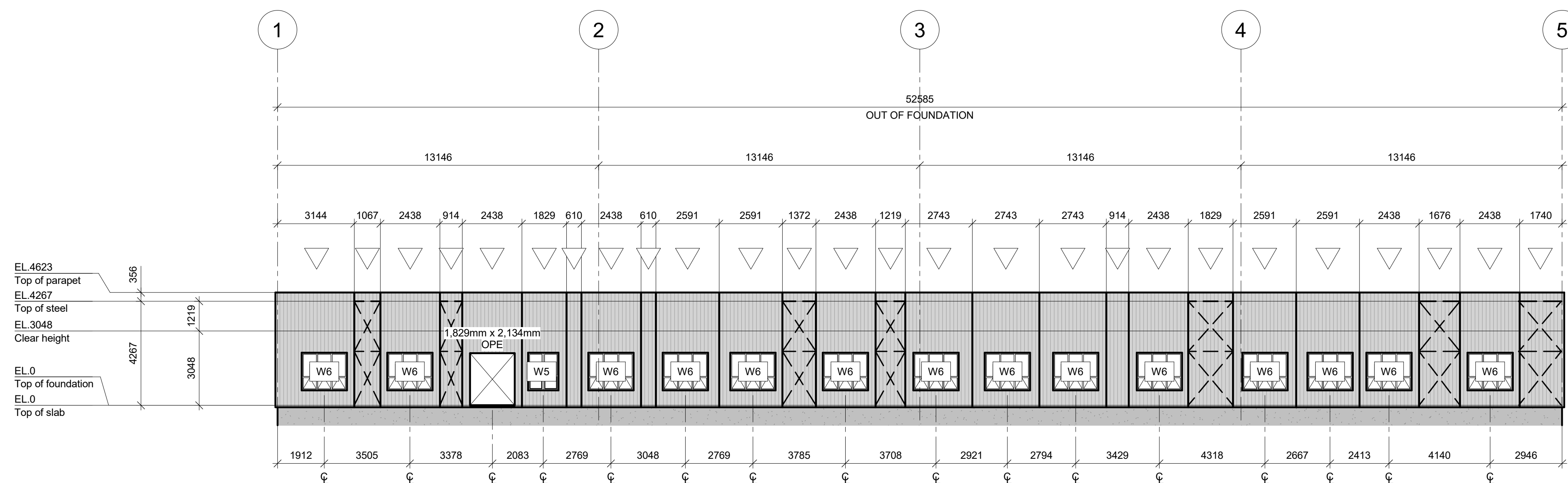
ELEVATION LINE A (SOUTH) 1 : 125
