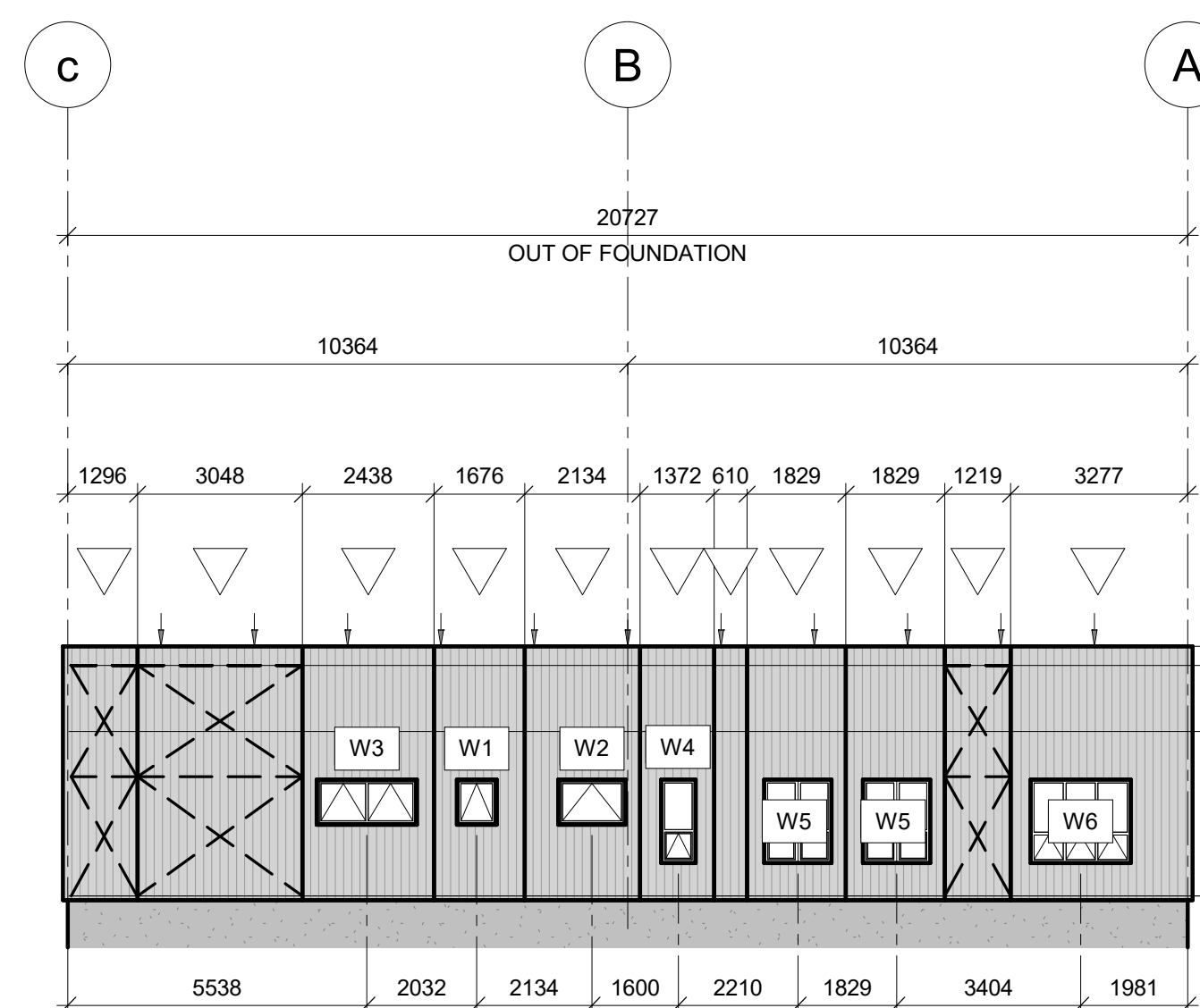
ELEVATION LINE 1 (WEST)
