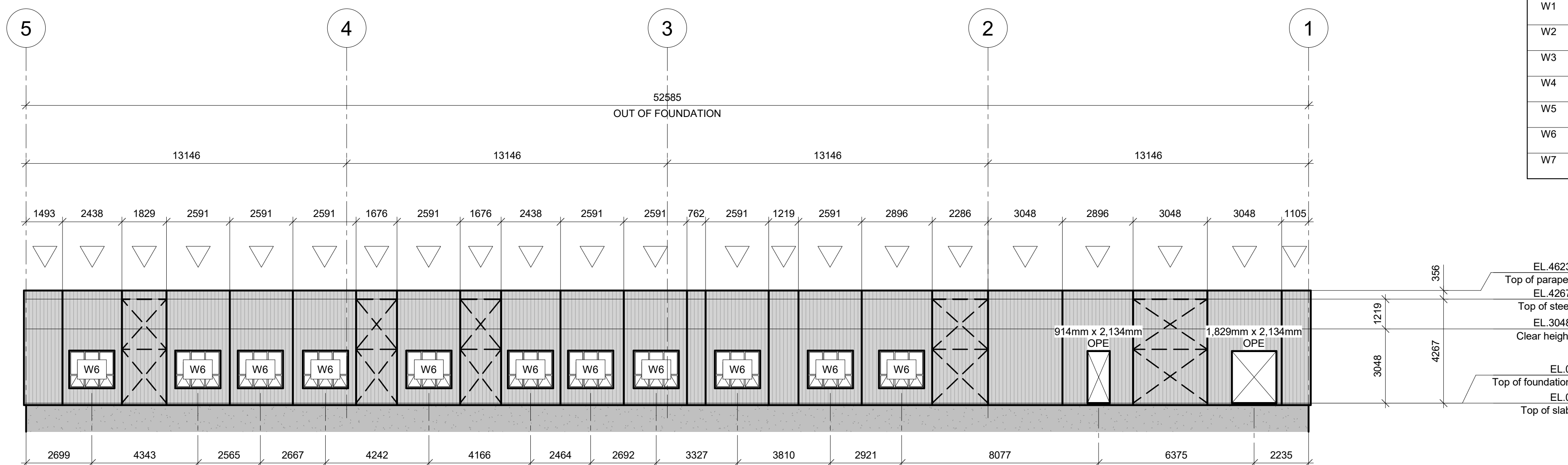
ELEVATION LINE C (NORTH) 1 : 125
