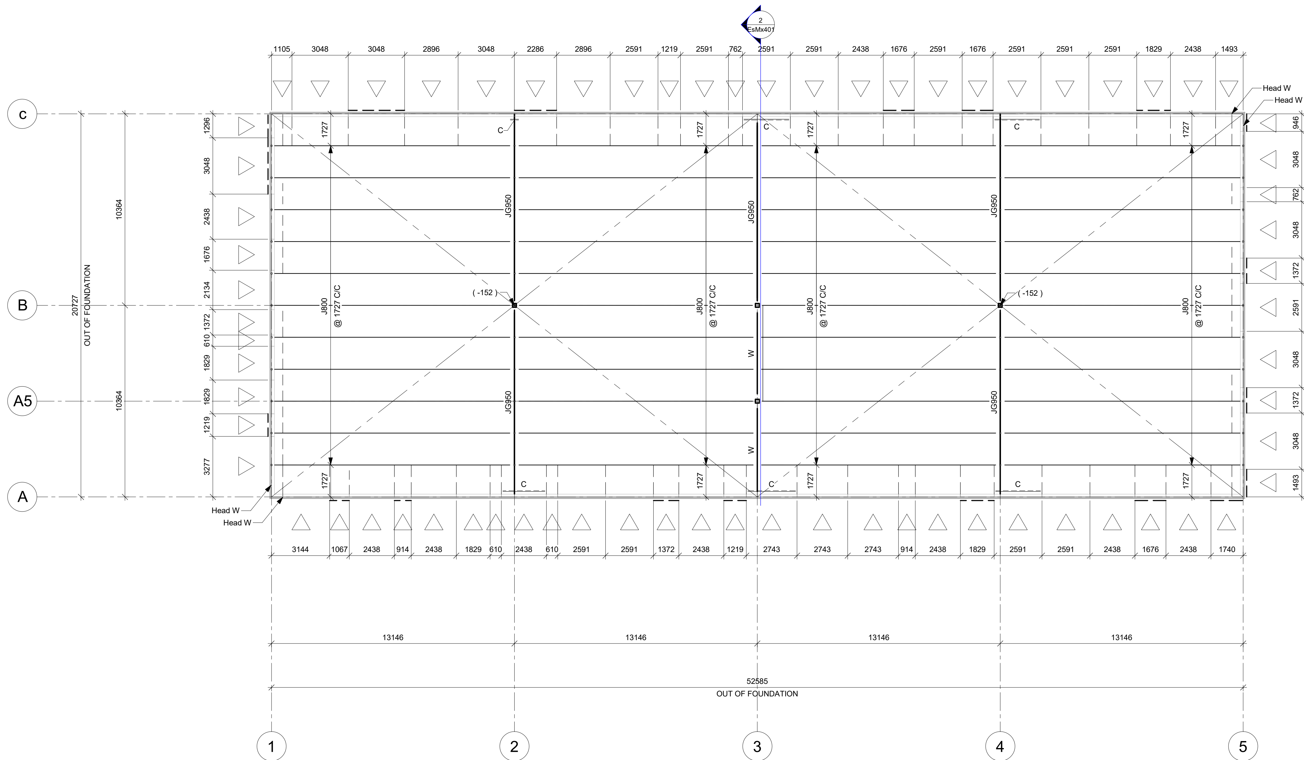
ROOF PLAN 1:125
