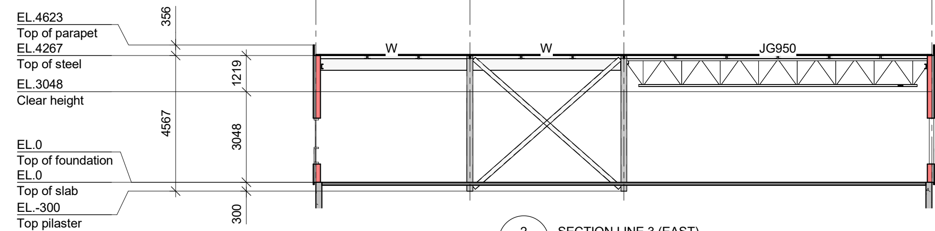
2 SECTION LINE 3 (EAST) EsMx401 1:125
