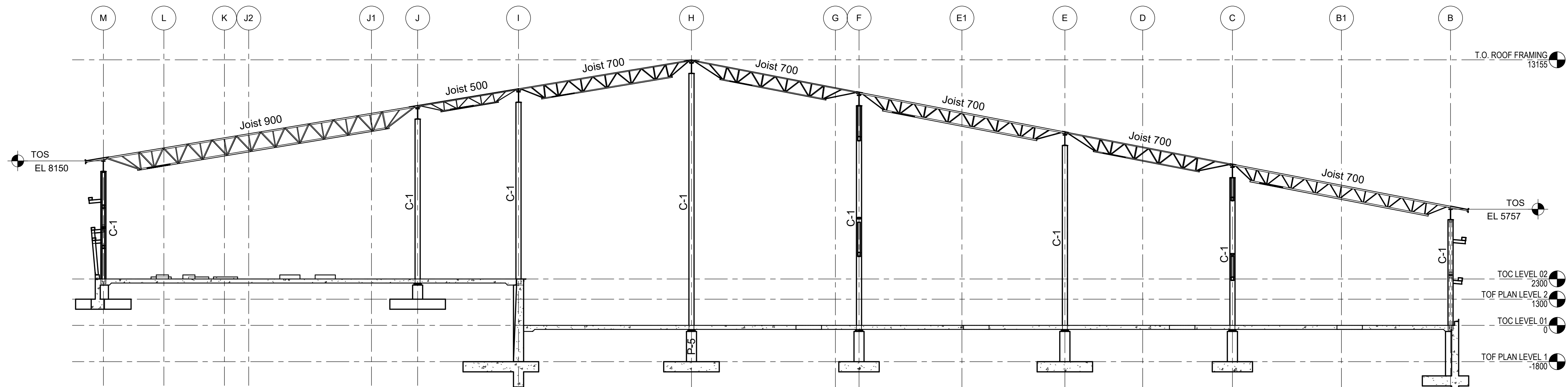
2 BUILDING SECTION (NEAR GL 8) S-101 1: 125
