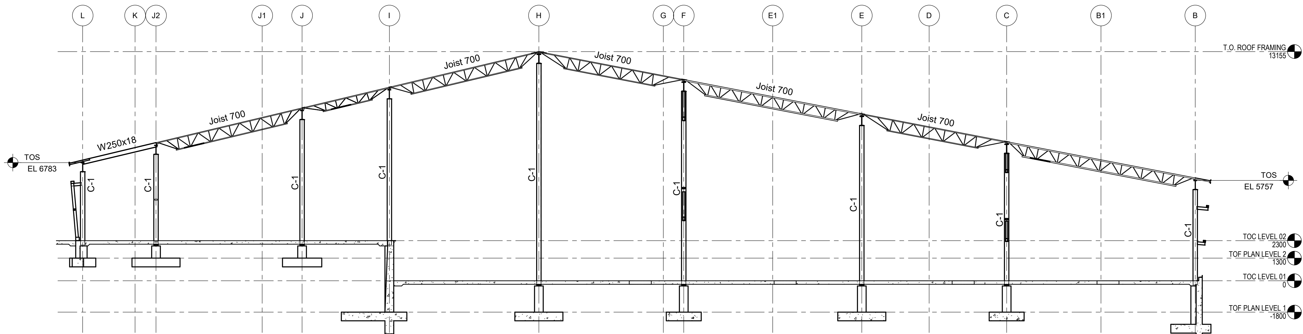
1 BUILDING SECTION (NEAR GL 4) S-101 1: 125
