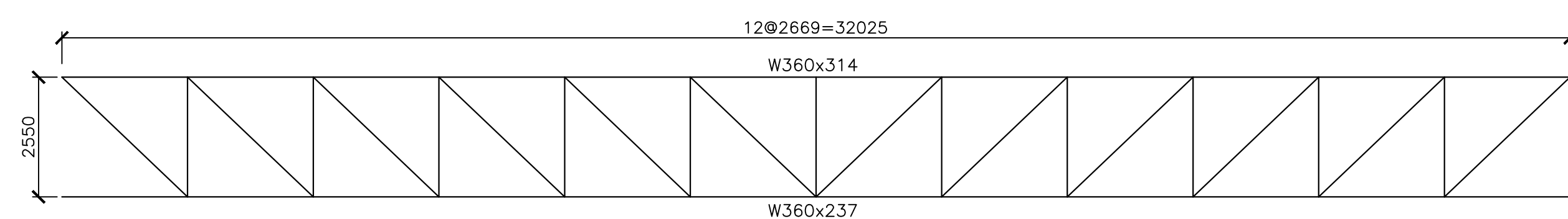
TRUSS TI VERTICAL MEMBERS : W200x46 UNO DIAGONAL MEMBERS : 2L152x203x13 UNO
