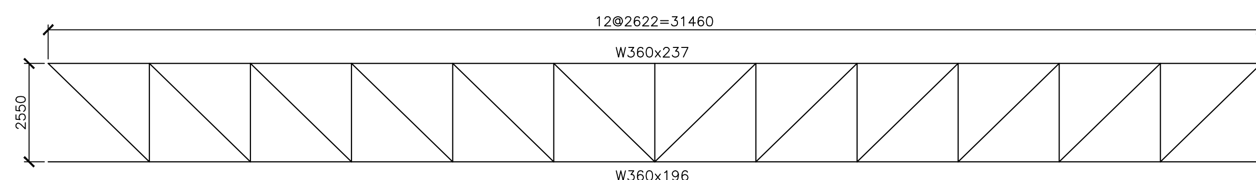
TRUSS T2 VERTICAL MEMBERS : W200x46 UNO DIAGONAL MEMBERS : 2L152x152x11 UNO
