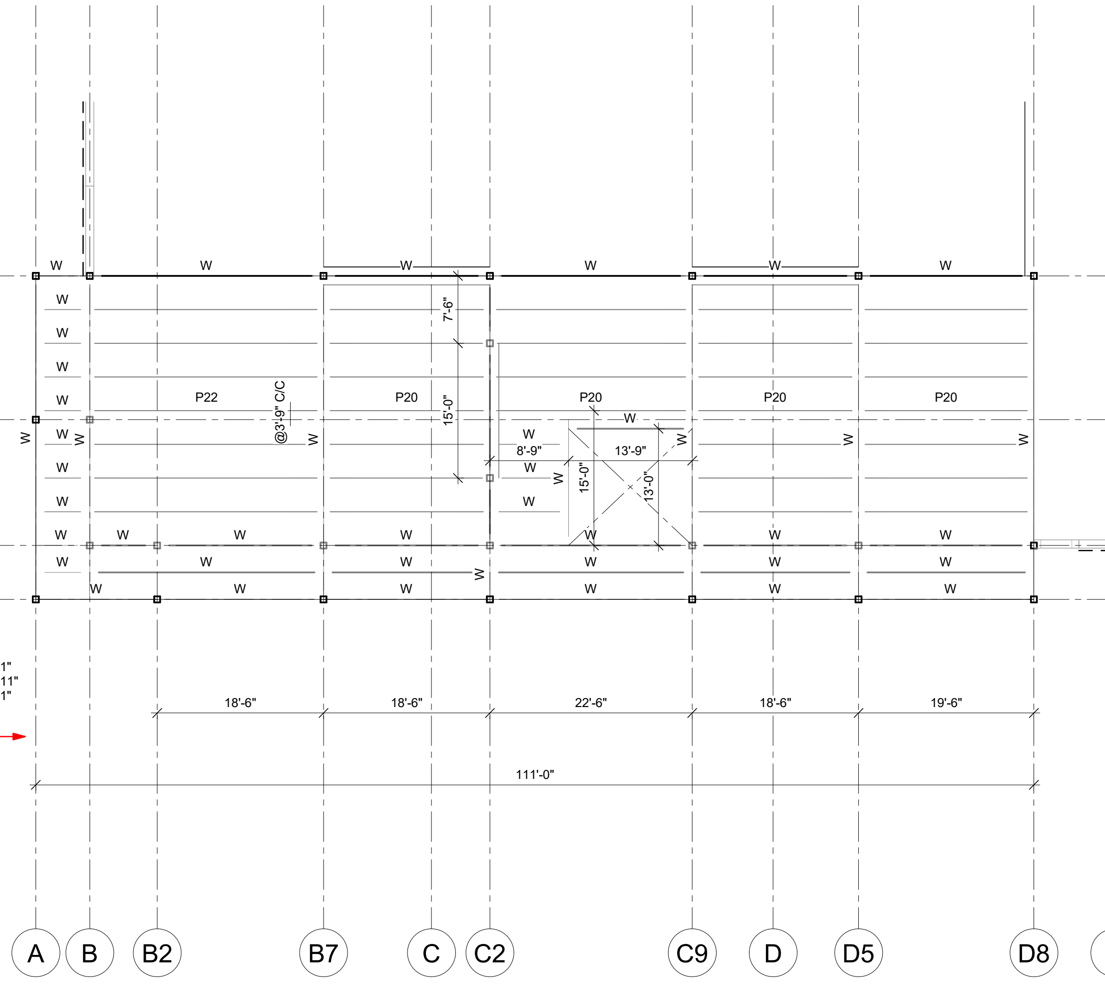
PLAN DE MEZZANINE 3/32" = 1'-0"
