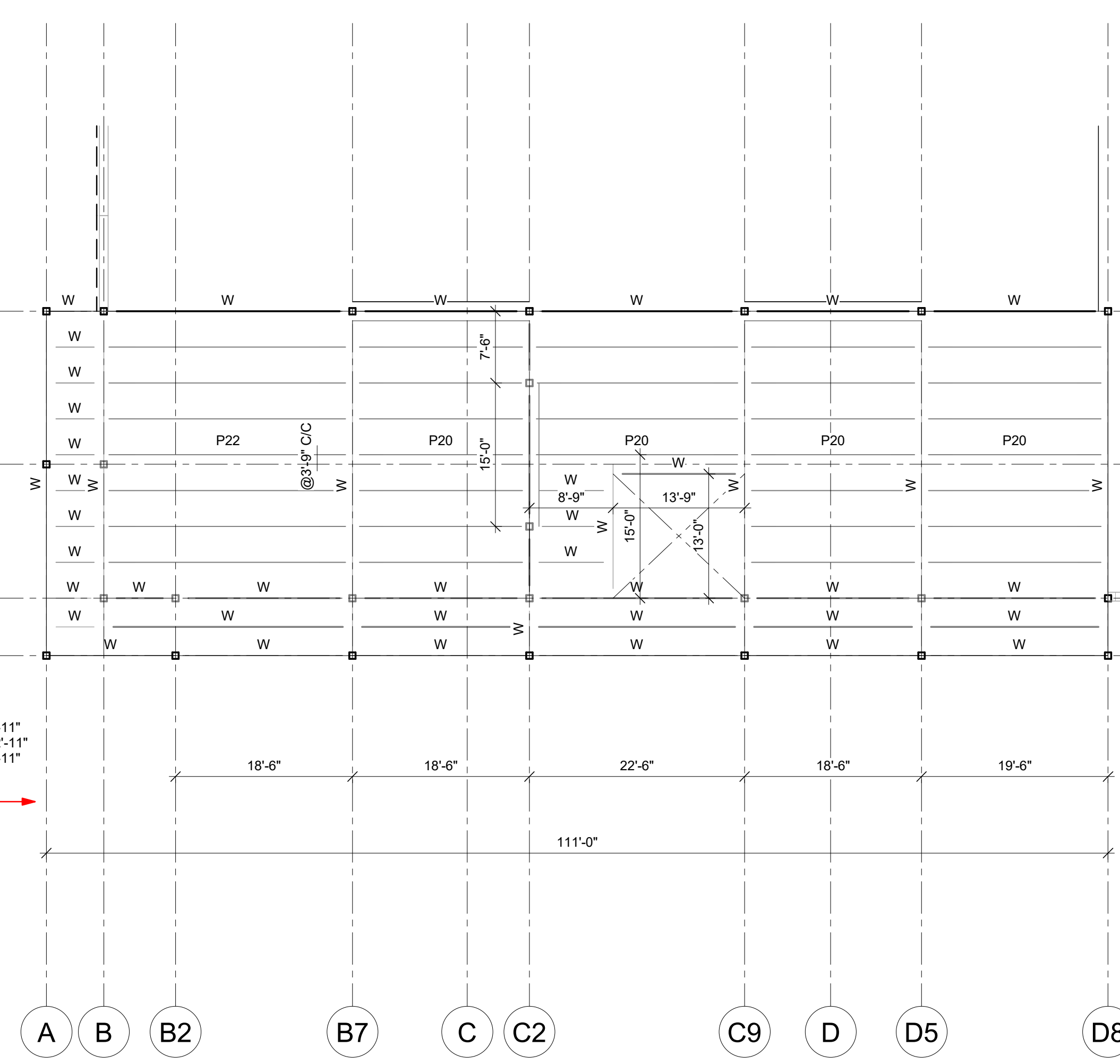
PLAN DE MEZZANINE 3/32" = 1'-0"
