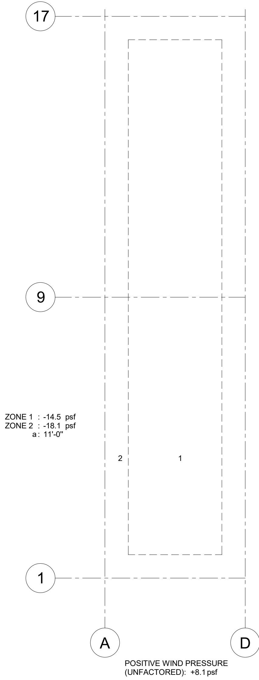
GROSS UPLIFT DIAGRAM (UNFACTORED):
