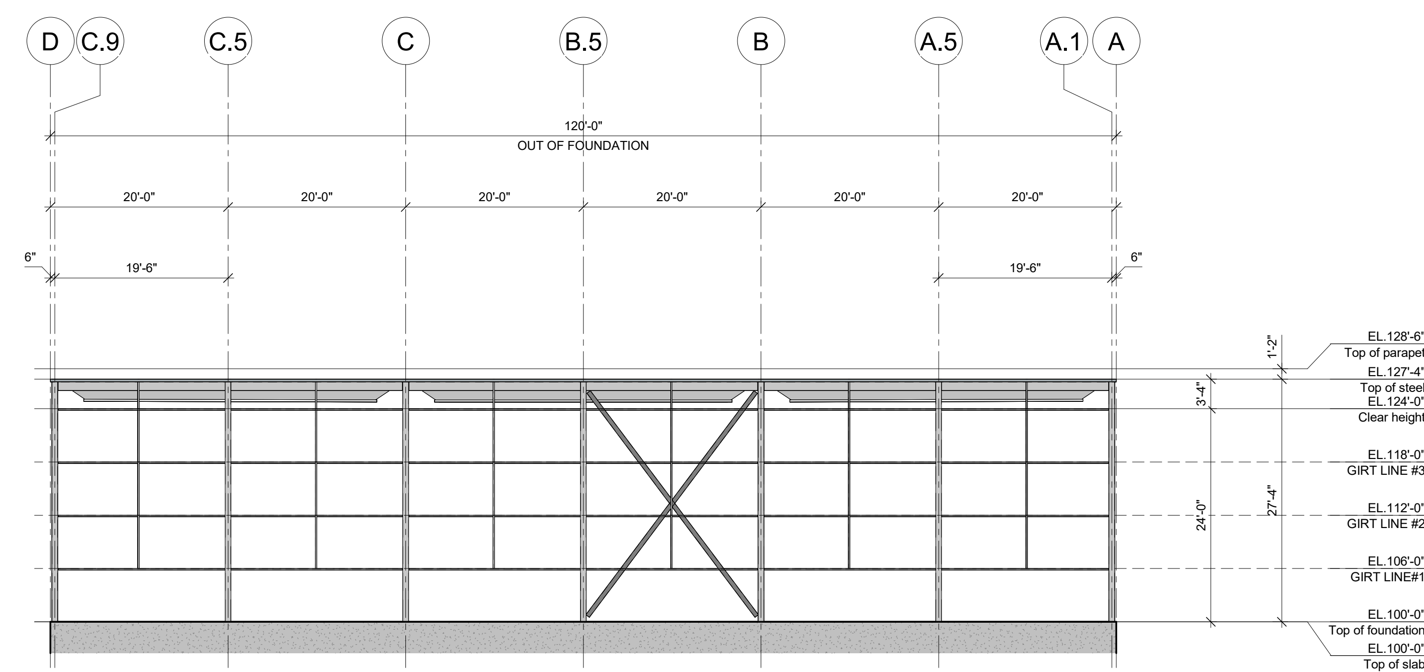
ELEVATION LINE 17 (NORTH) 3/32" = 1'-0"
