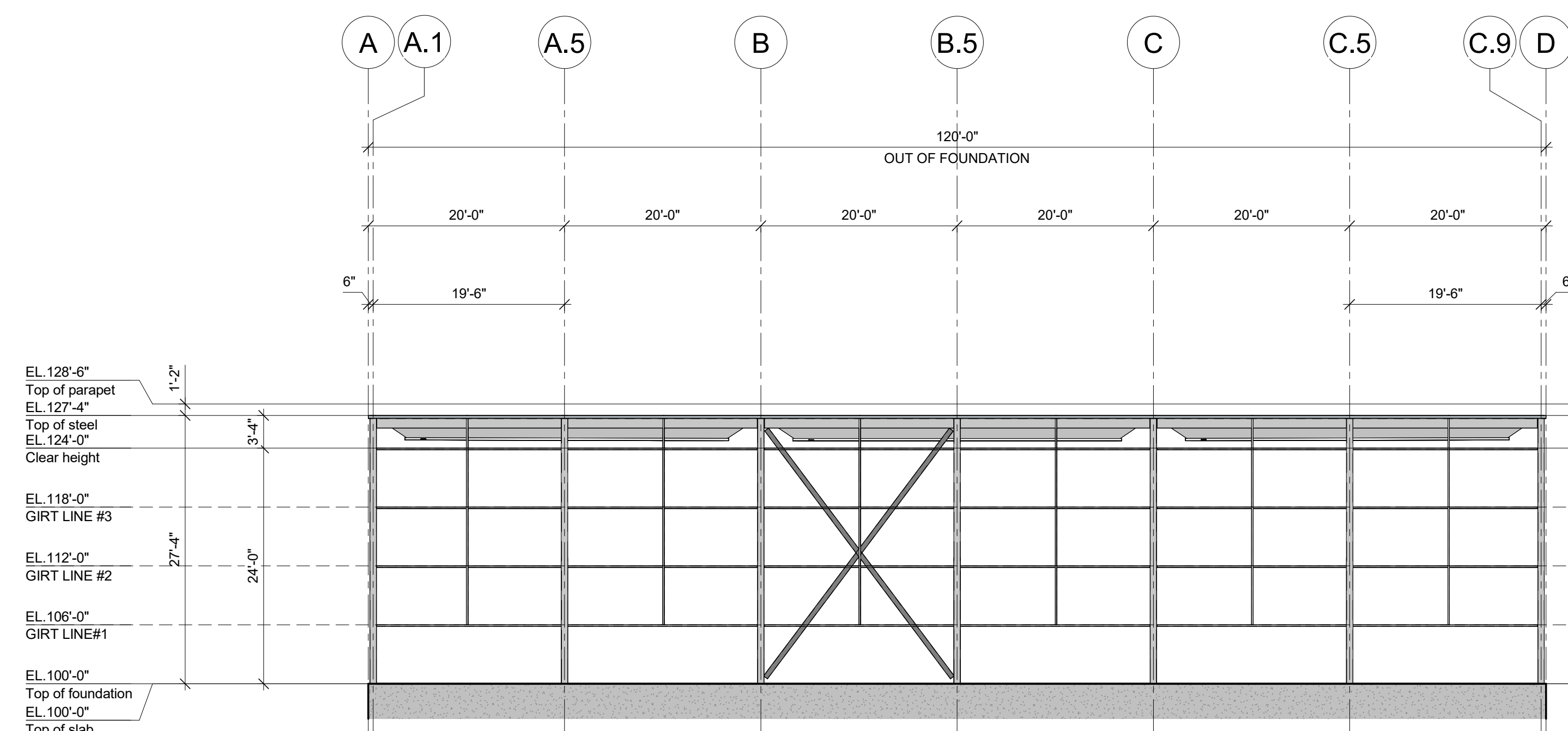
ELEVATION LINE 1 (SOUTH) 3/32" = 1'-0"
