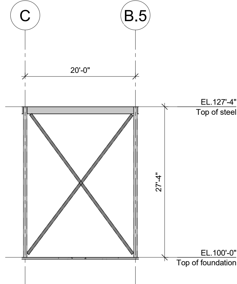
BRACING ELEVATION LINE 9.1 3/32" = 1'-0"
