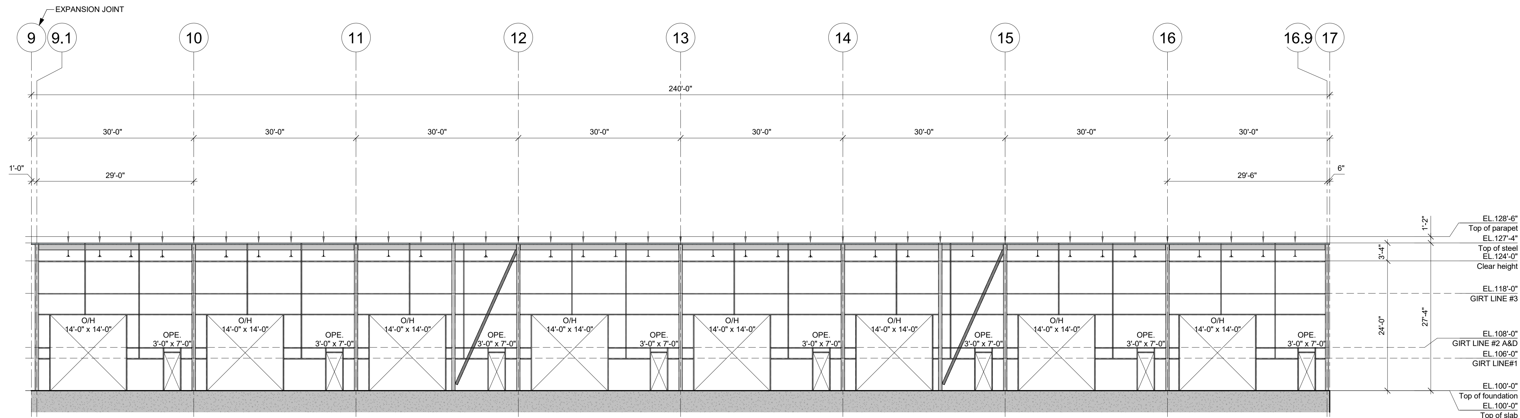
ELEVATION LINE D (EAST) - LINE 9 @ 17 3/32" = 1'-0"
