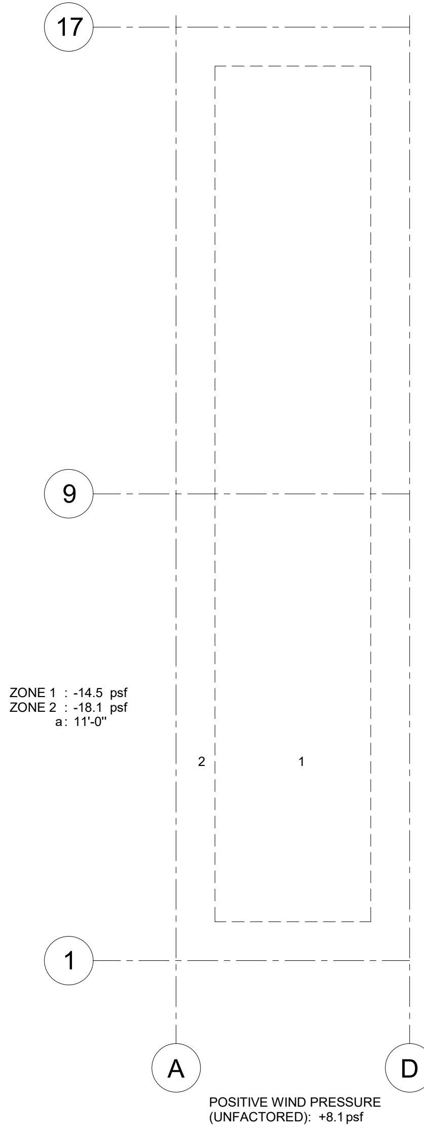
GROSS UPLIFT DIAGRAM (UNFACTORED):
