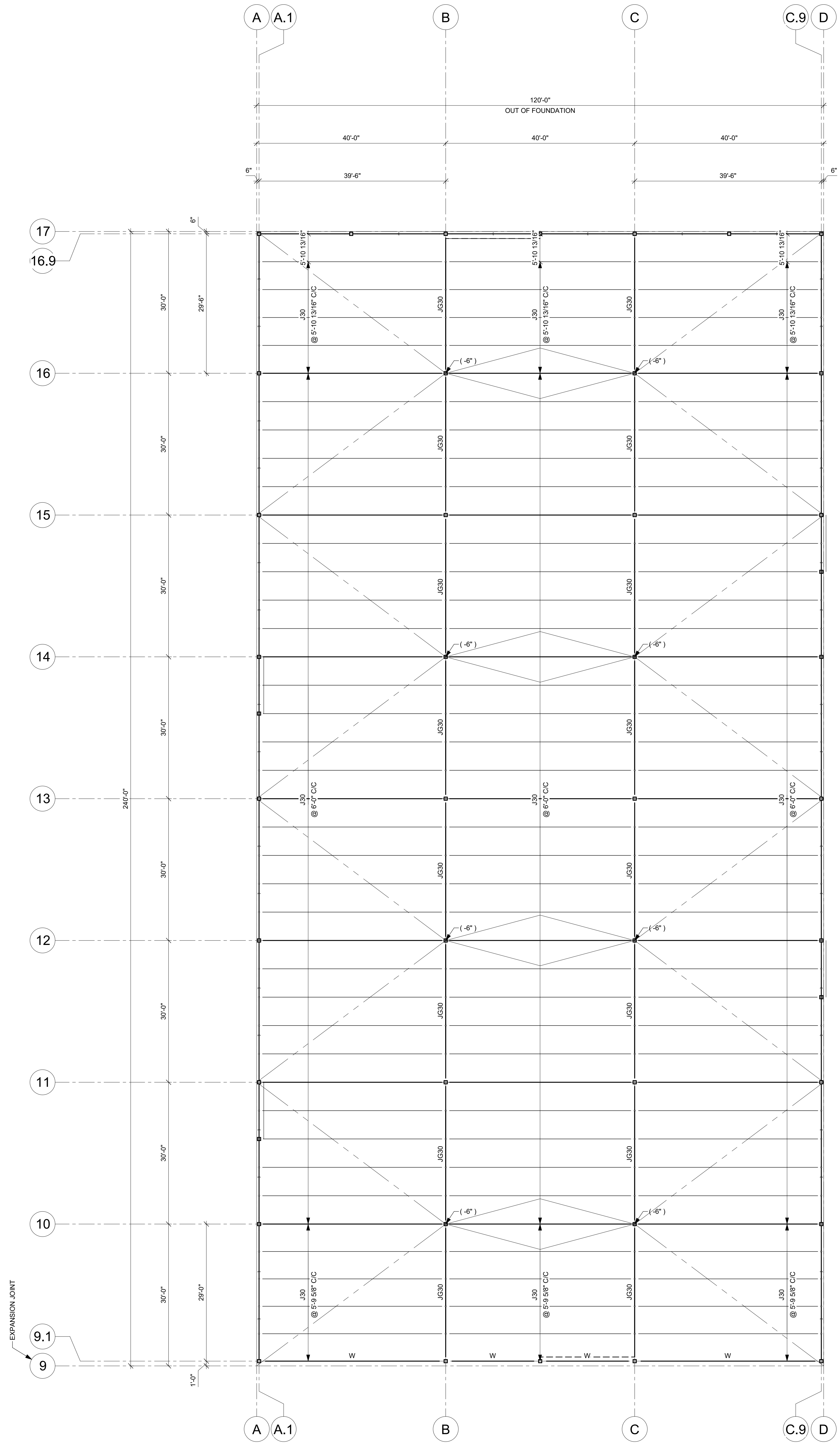
ROOF PLAN - LINE 9 @ 17 3/32" = 1'-0"
