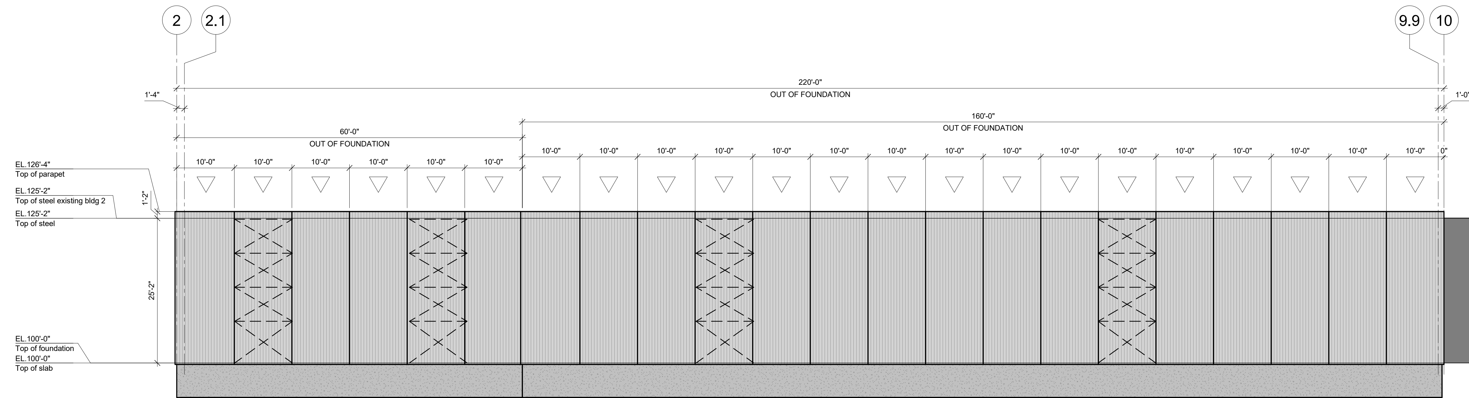
ELEVATION LINE S.6 & T (EAST) 1" = 10'-0"
