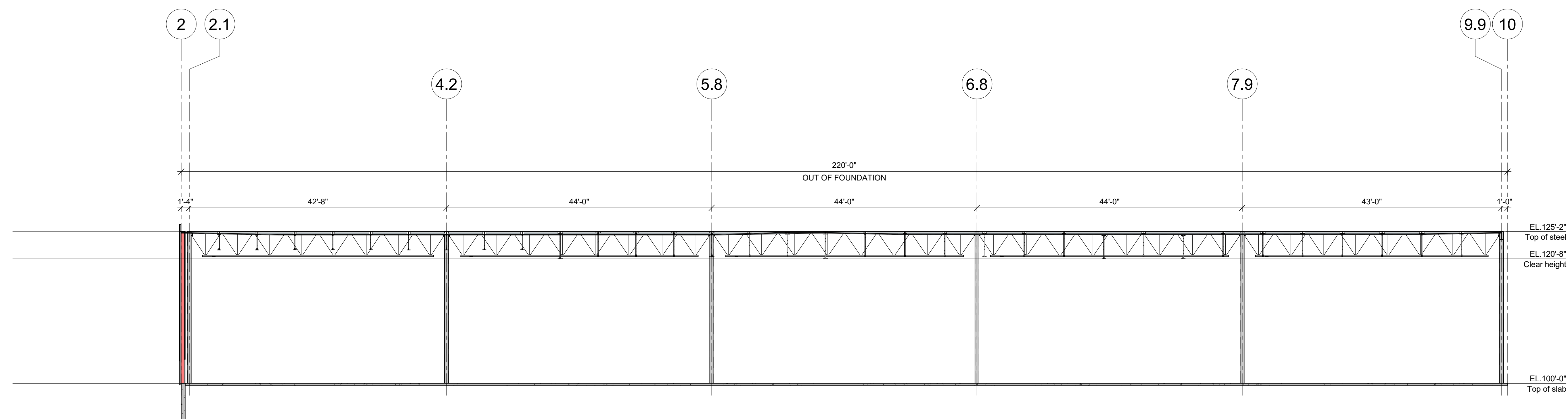
ELEVATION LINE R.7 (STRUCTURE) (EAST) 1" = 10'-0"
