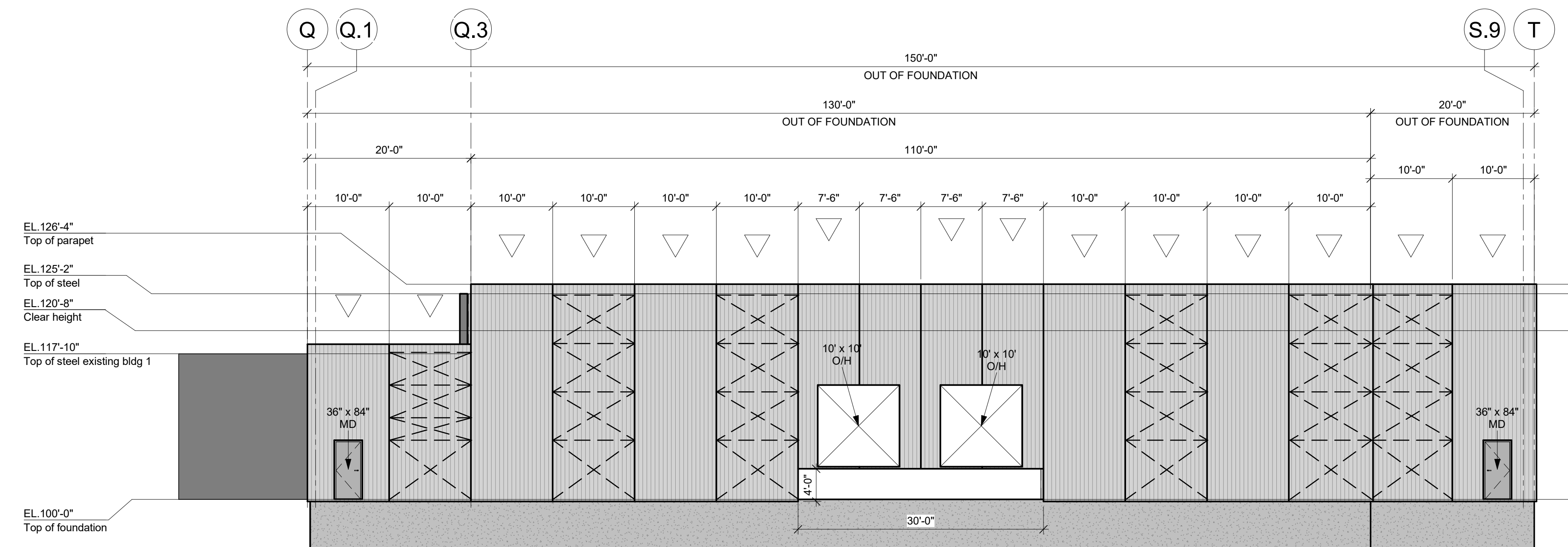
ELEVATION LINE 2 (SOUTH) 1" = 10'-0"
