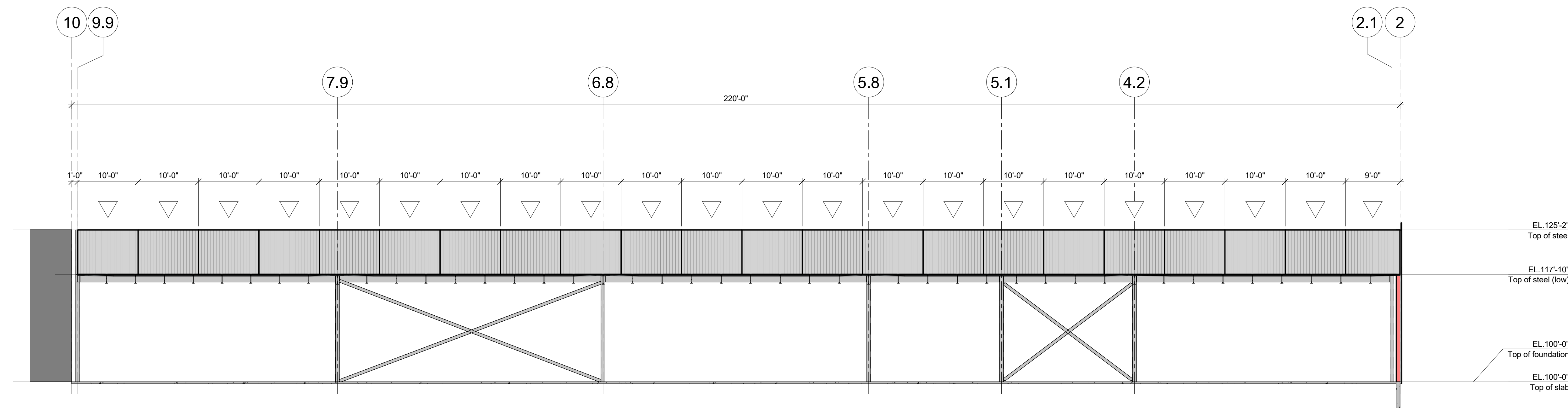
ELEVATION LINE Q.3 (HIGH & LOW PANELS)(WEST) 1" = 10'-0"
