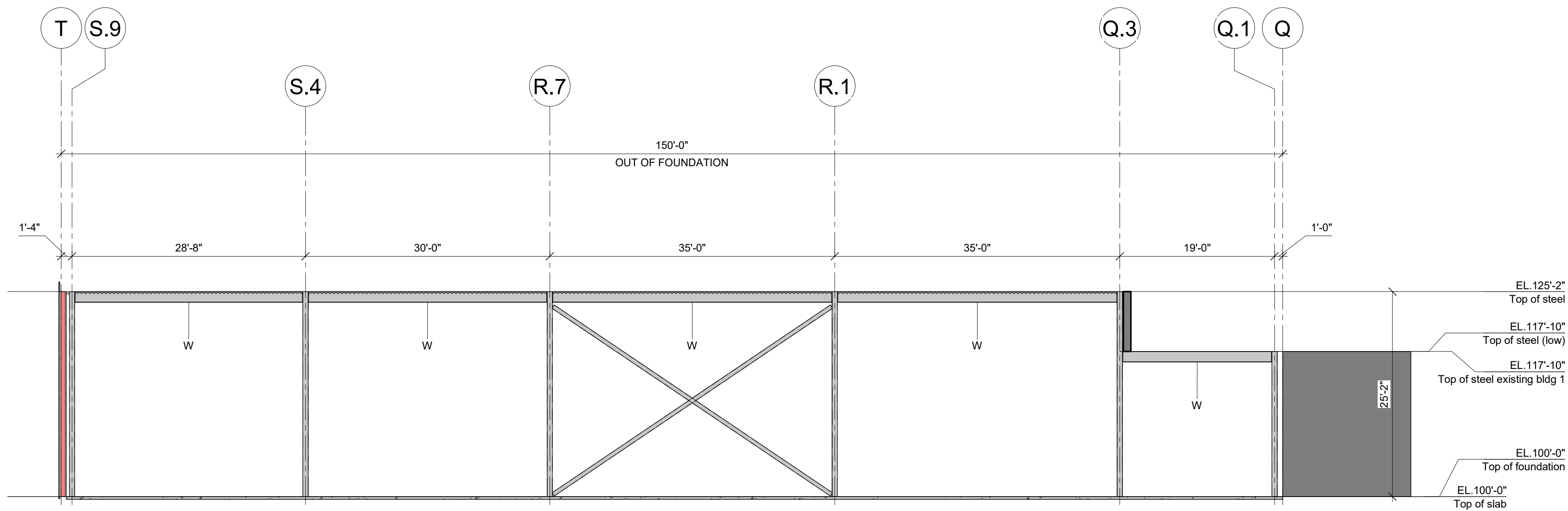
ELEVATION LINE 9.9 (STRUCTURE) (NORTH) 1" = 10'-0"
