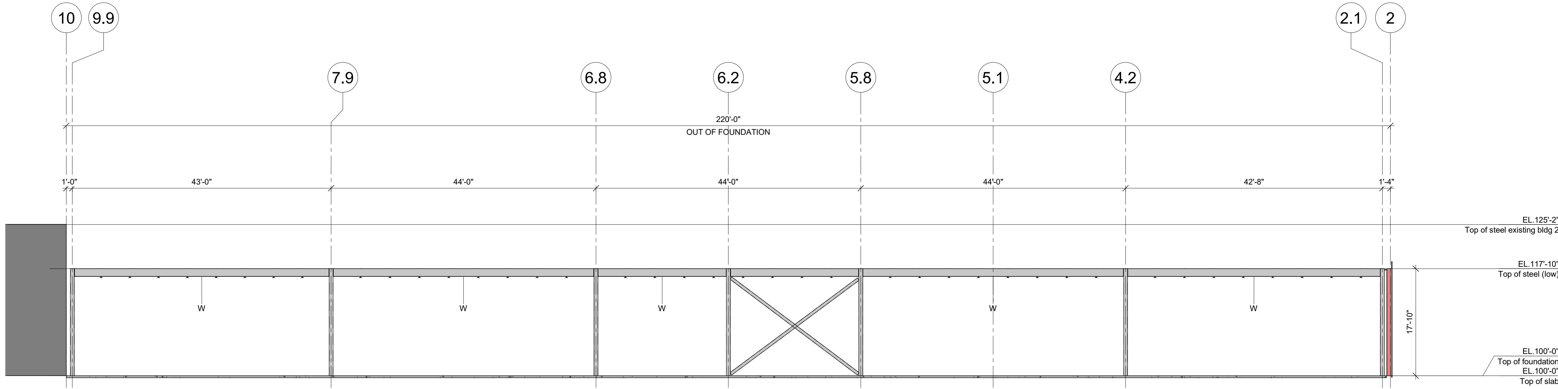
ELEVATION LINE Q (STRUCTURE)(WEST) 1" = 10'-0"
