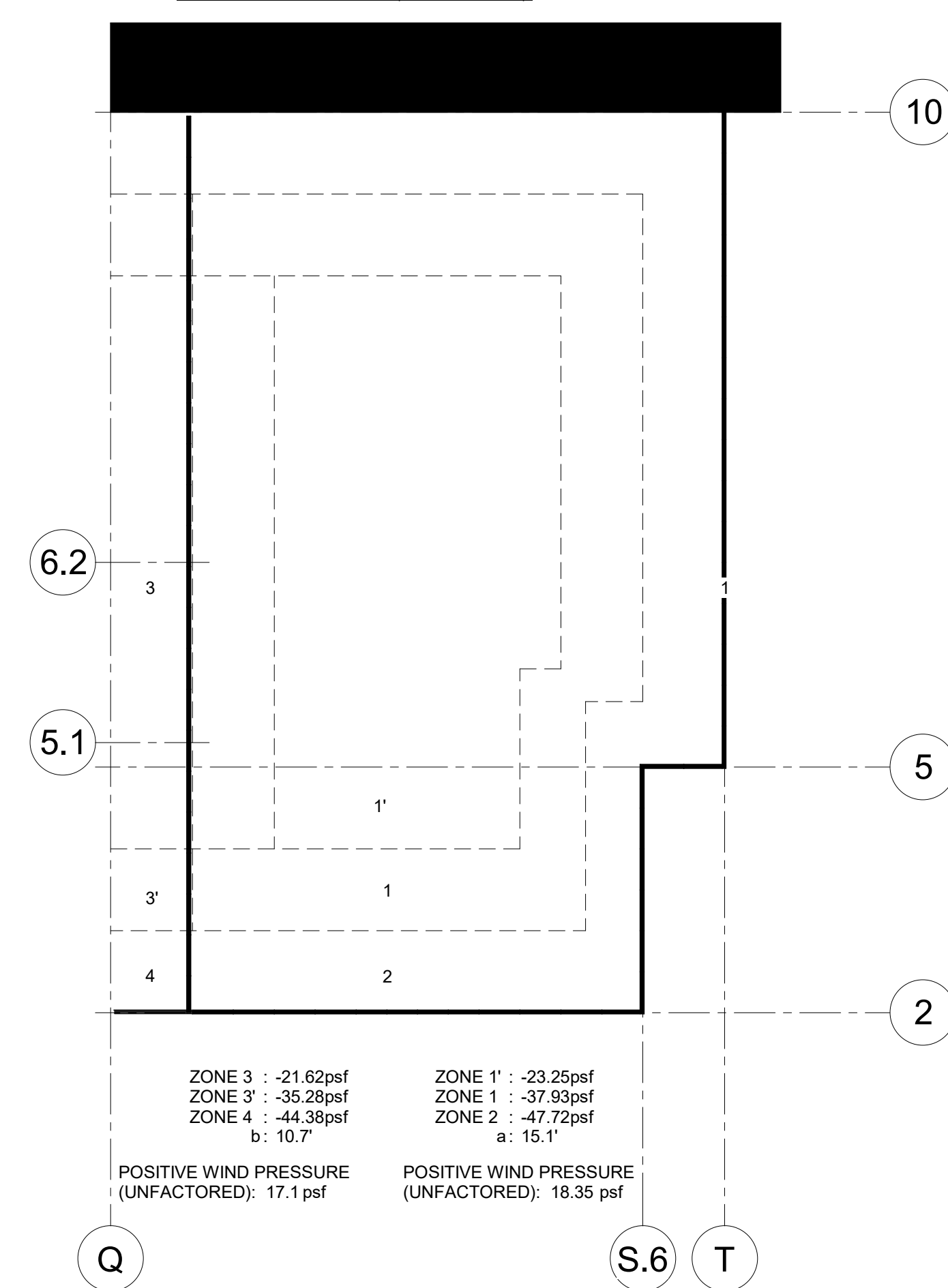
GROSS UPLIFT DIAGRAM (UNFACTORED)
