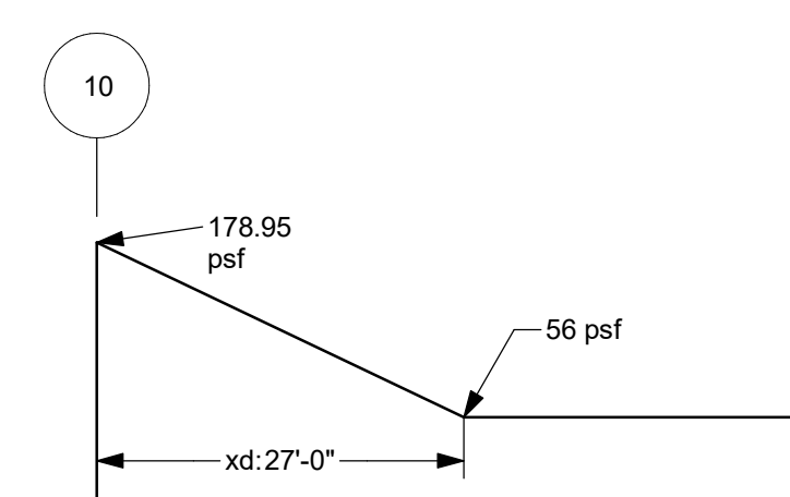
SNOW LOAD ACCUMULATION
