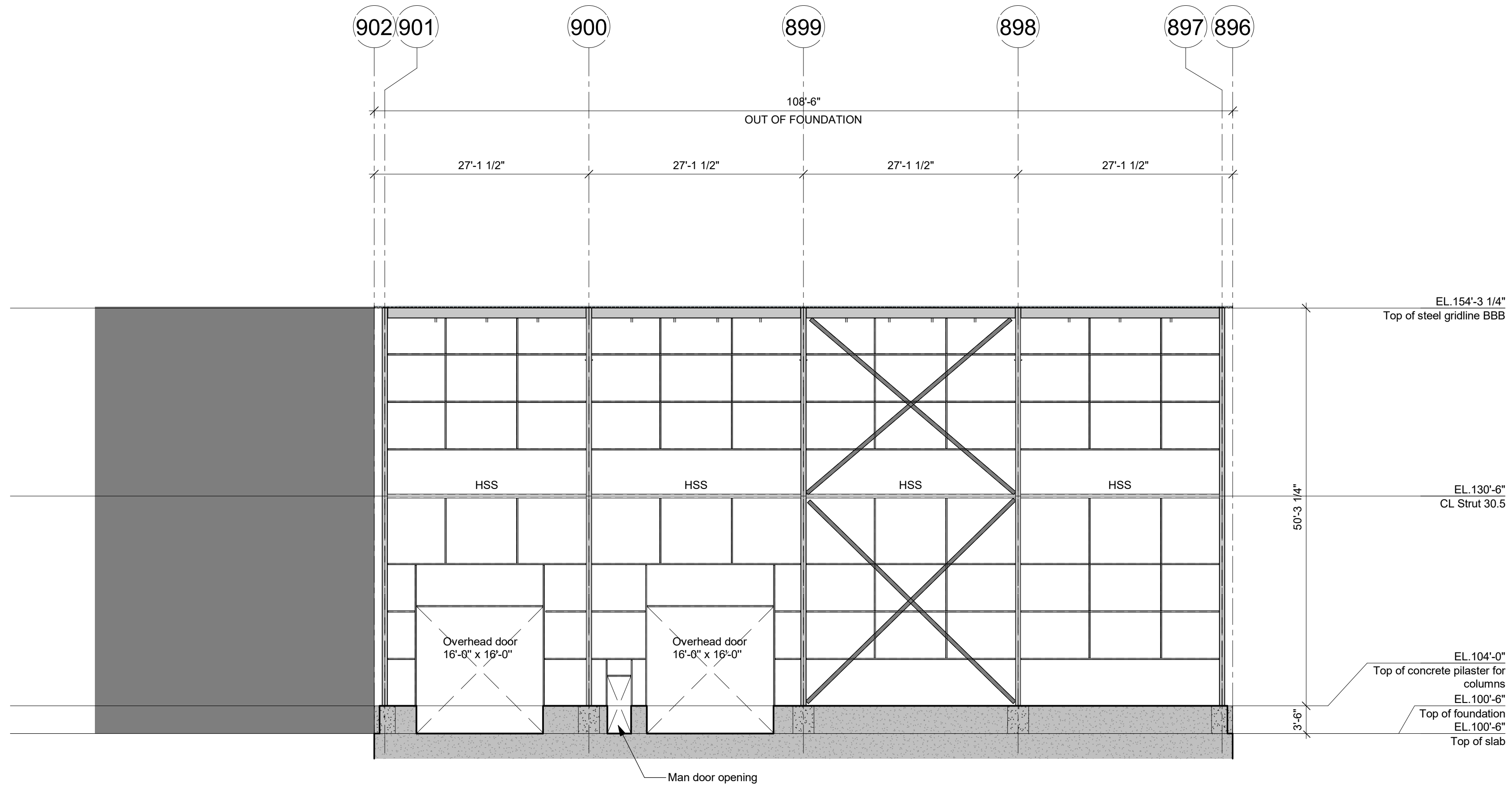
ELEVATION LINE BBB (WEST) 3/32" = 1'-0"
