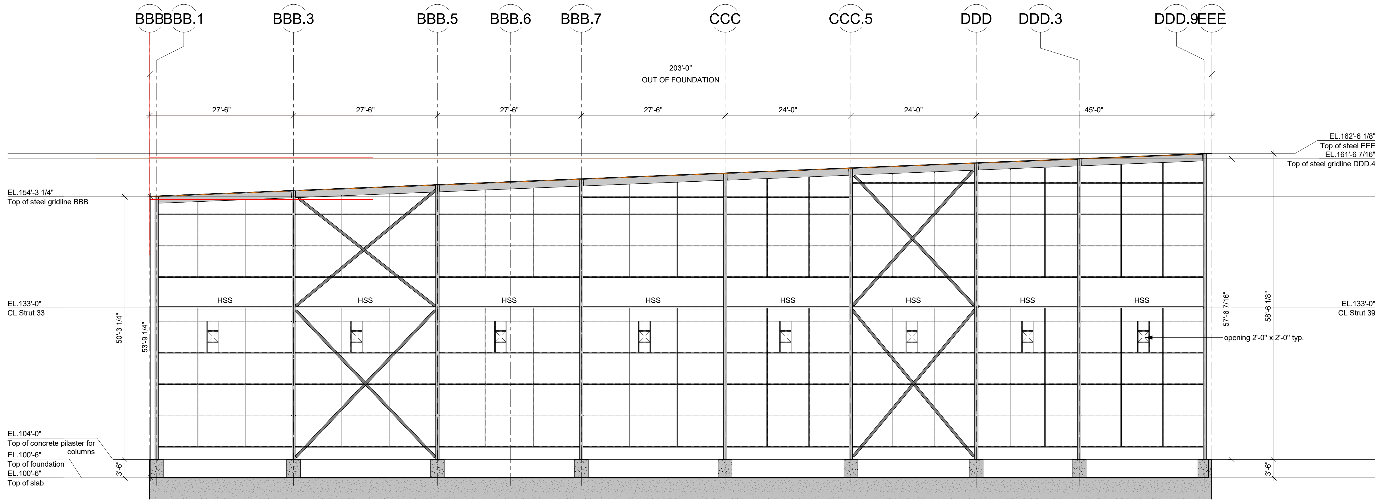
ELEVATION LINE 902 (SOUTH) 3/32" = 1'-0"
