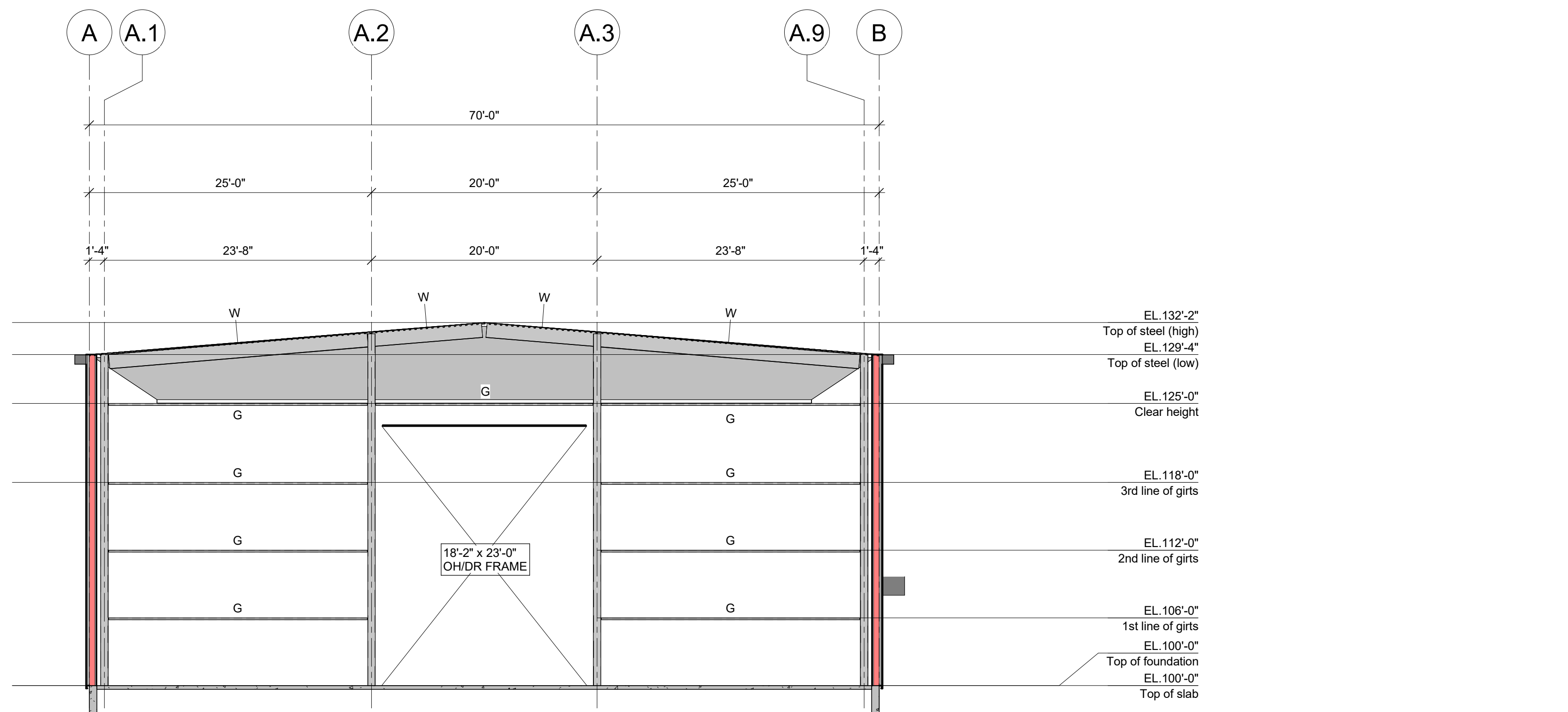
ELEVATION LINE 2.4 (WEST)(STRUCTURE) 1/8" = 1'-0"
