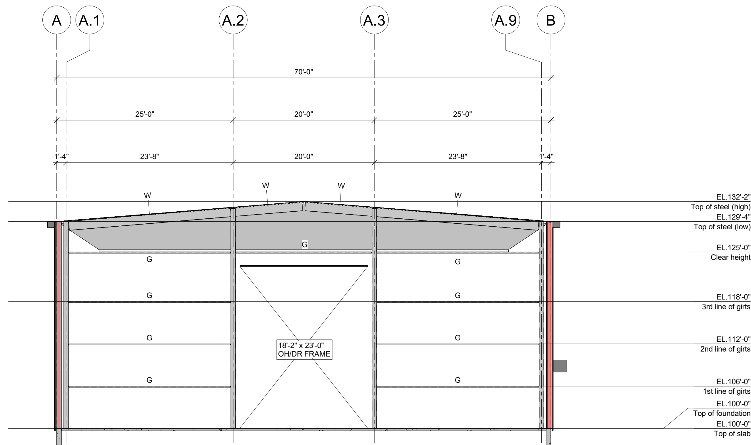
ELEVATION LINE 2.4 (WEST)(STRUCTURE) 1/8" = 1'-0"
