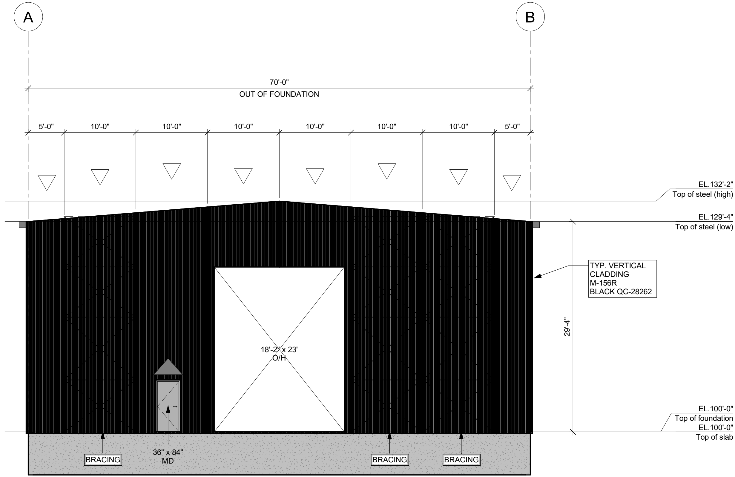
ELEVATION LINE 3 (WEST) 1/8" = 1'-0"
