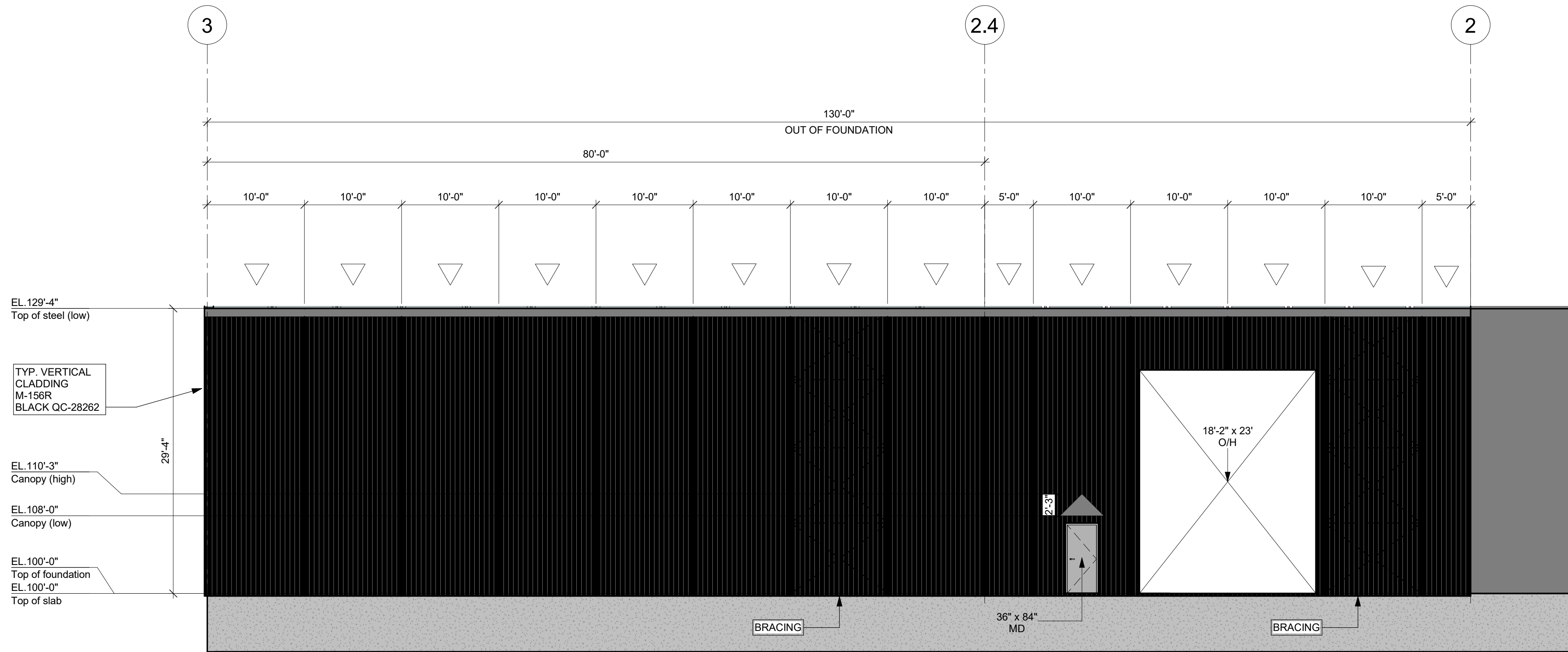
ELEVATION LINE B (SOUTH) 1/8" = 1'-0"
