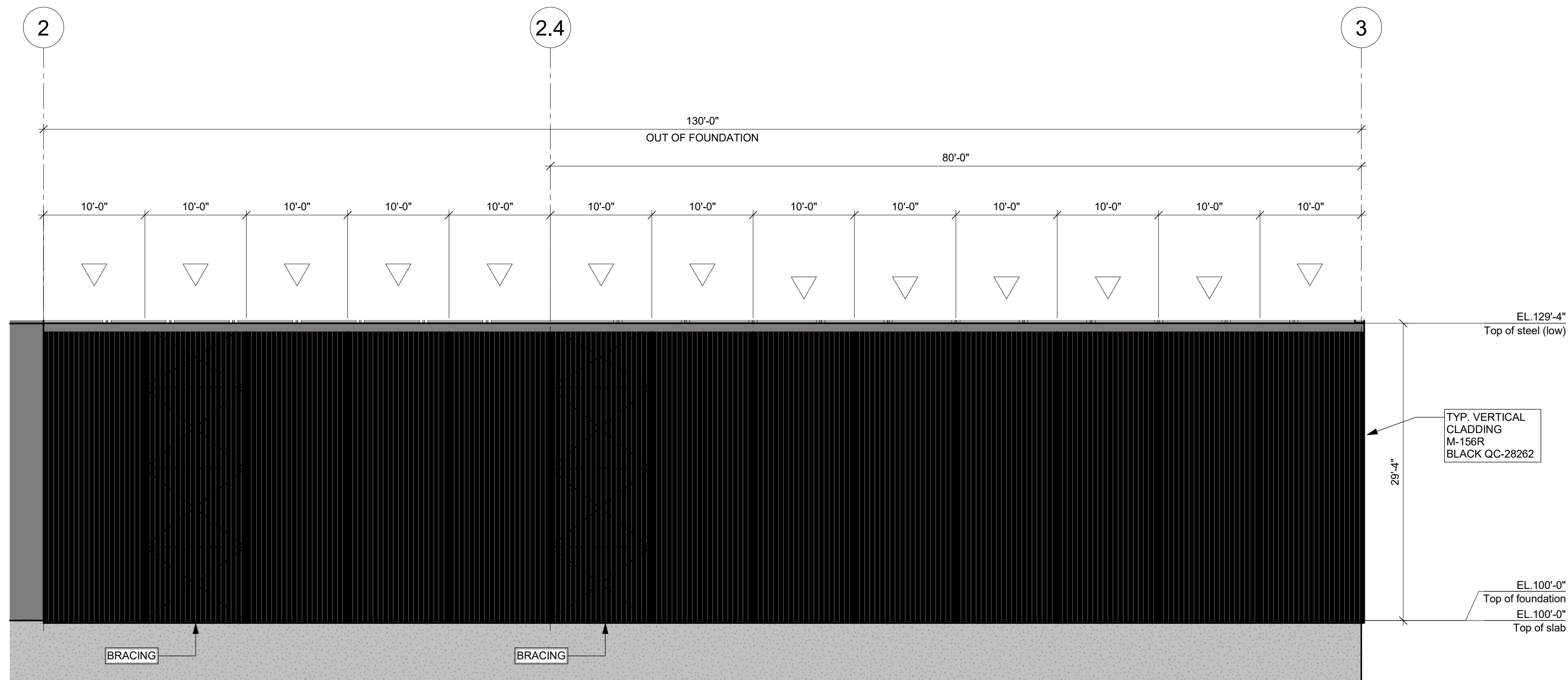
ELEVATION LINE A (NORTH) 1/8" = 1'-0"
