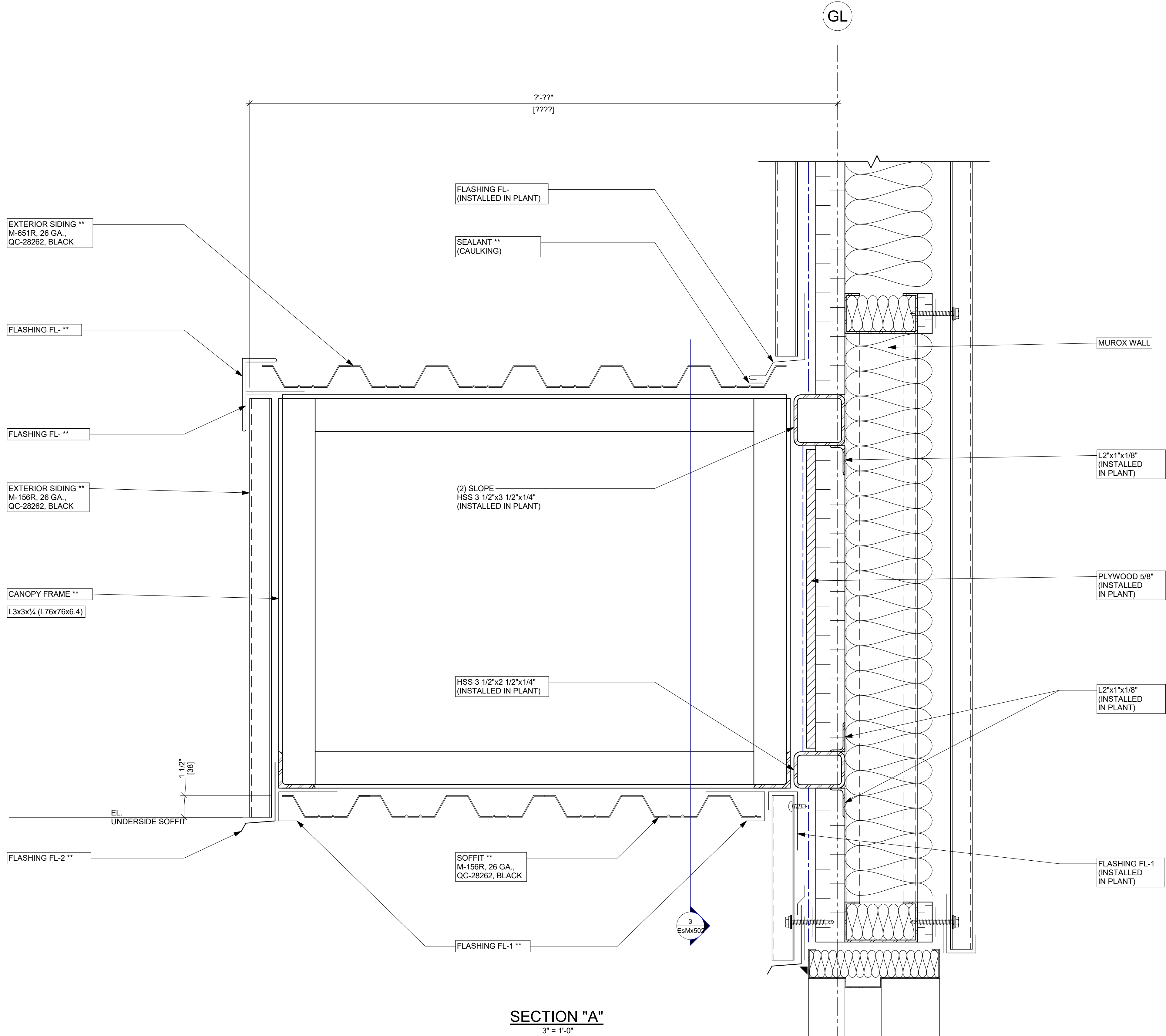
SECTION "A" 3" = 1'-0"
