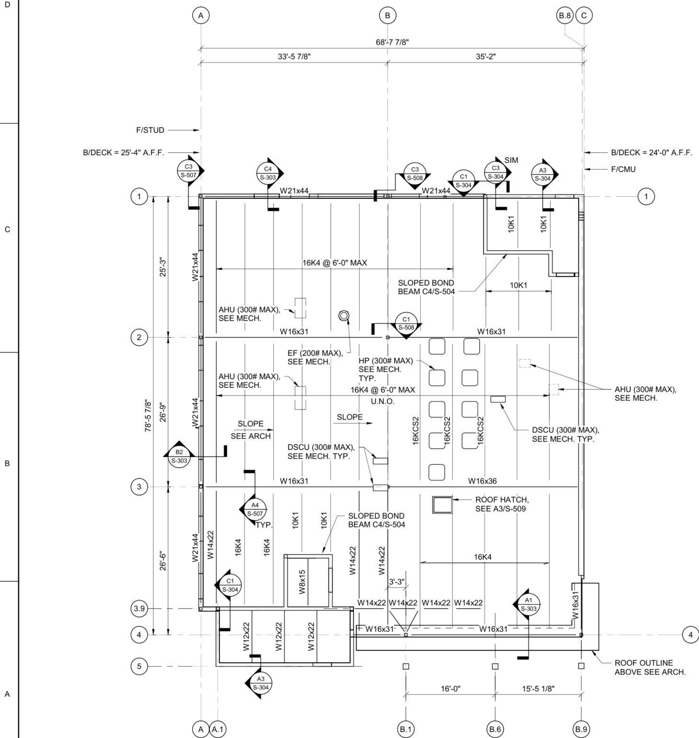
A1 ROOF FRAMING PLAN SCALE: 1/8" = 1'-0"
