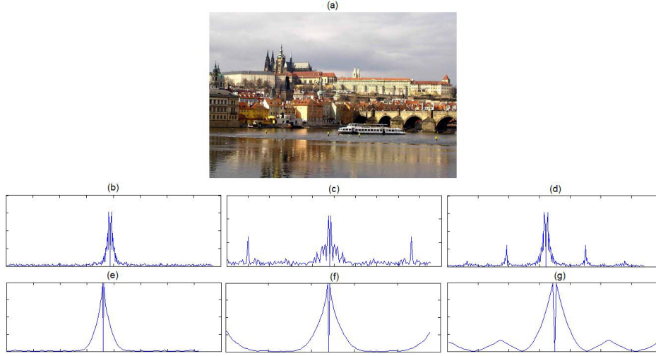
Figure 2: In (a) the test image is shown. (b) and (e) show the magnitudes of Fourier transform of the zero-mean histograms of DCT coefficients corresponding to frequencies (0, 0) and (1, 1) obtained from a single compressed version of (a). Here the image was saved by quality factor 85. (c) and (f) show the same for the double compressed version of (a). Here the image was saved by quality factor 85 followed by quality factor 75. (d) and (g) show the same for double compressed version of (a) with quality factor 85 followed by quality factor 80.
