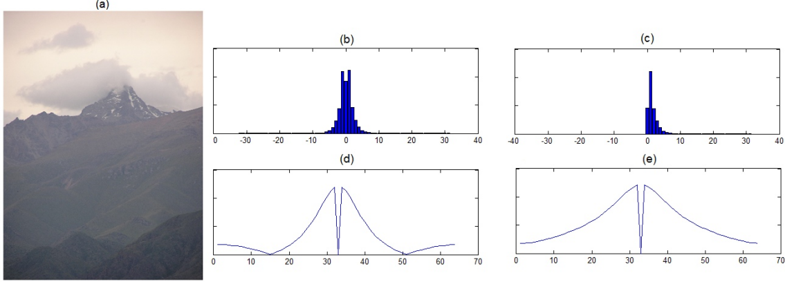
Figure 3: Shown are: (a) the tested single compressed images; (b),(d) outputs of the method described in [13] resulting in a false positive (the spectrum has not the typical decaying trend); (c),(e) output of the method described in this paper. In both cases the method was applied to DCT coefficients corresponding to frequency (1, 0).
