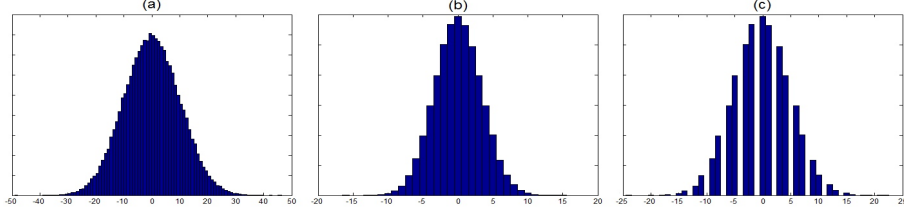
Figure 1: Shown are: (a) the histogram of a non-quantized random values drawn from a zero-mean normal distribution; (b) histogram of the quantized (a) with quantization step Q^\alpha = 3 ; (c) histogram of the double-quantized (a) with quantization steps Q^\alpha = 3 and Q^\beta = 2 .
