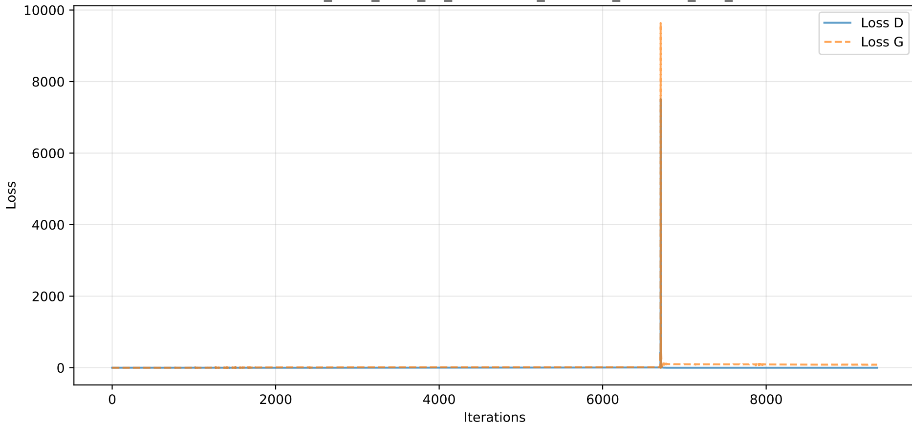
Losses - e20_b128_z100_k1_Oadabelief_lrG0.002_lrD0.002_l0.9_S42
