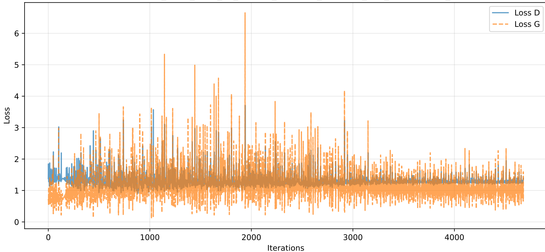
Losses - e20_b256_z100_k1_Oadam_lrG0.002_lrD0.002_l0.9_be0.5-0.999_S42
