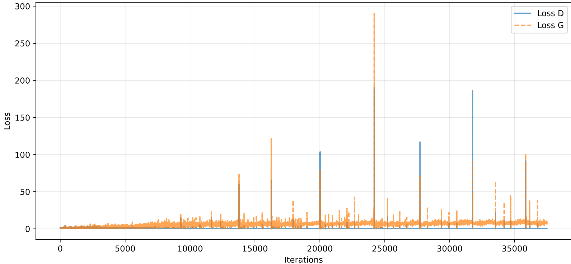
Losses - e20_b32_z100_k1_Oadam_lrG0.002_lrD0.002_l0.9_be0.5-0.999_S42
