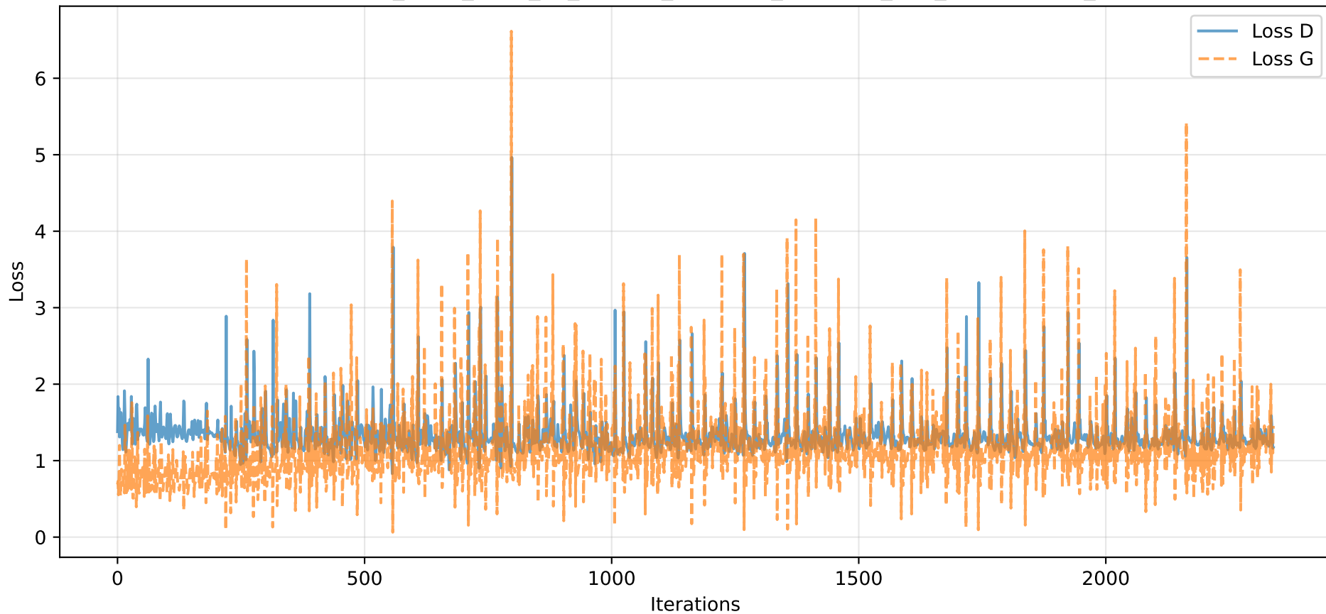
Losses - e20_b512_z100_k1_Oadam_lrG0.002_lrD0.002_l0.9_be0.5-0.999_S42
