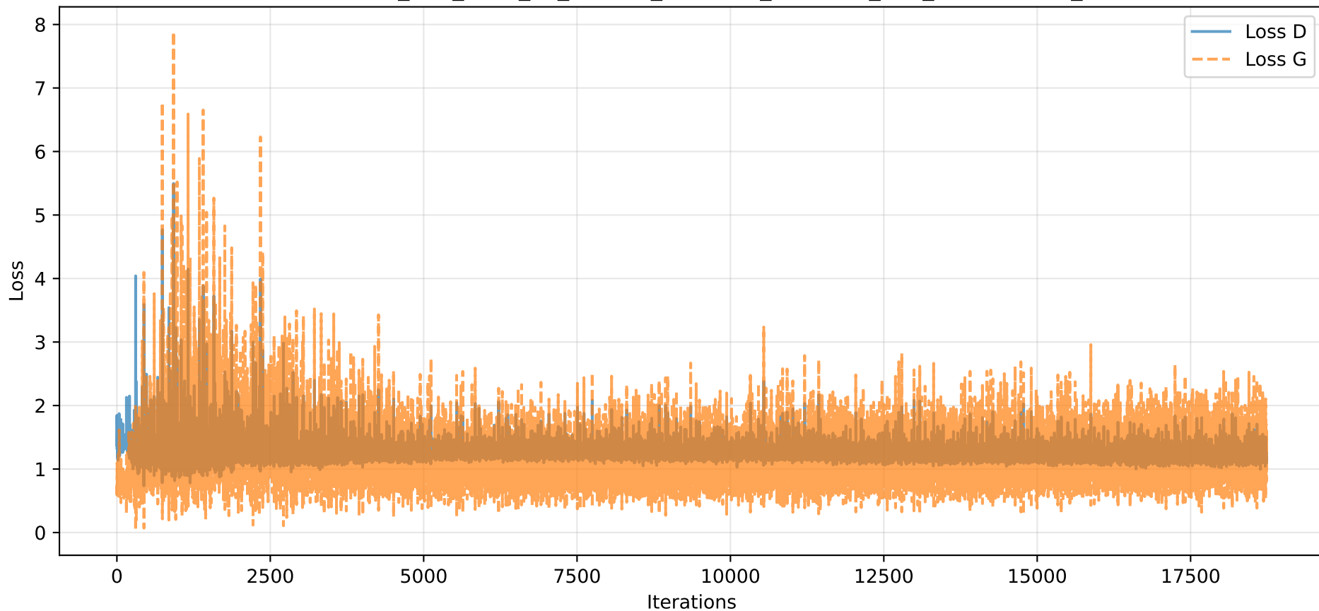
Losses - e20_b64_z100_k1_Oadam_lrG0.002_lrD0.002_l0.9_be0.5-0.999_S42
