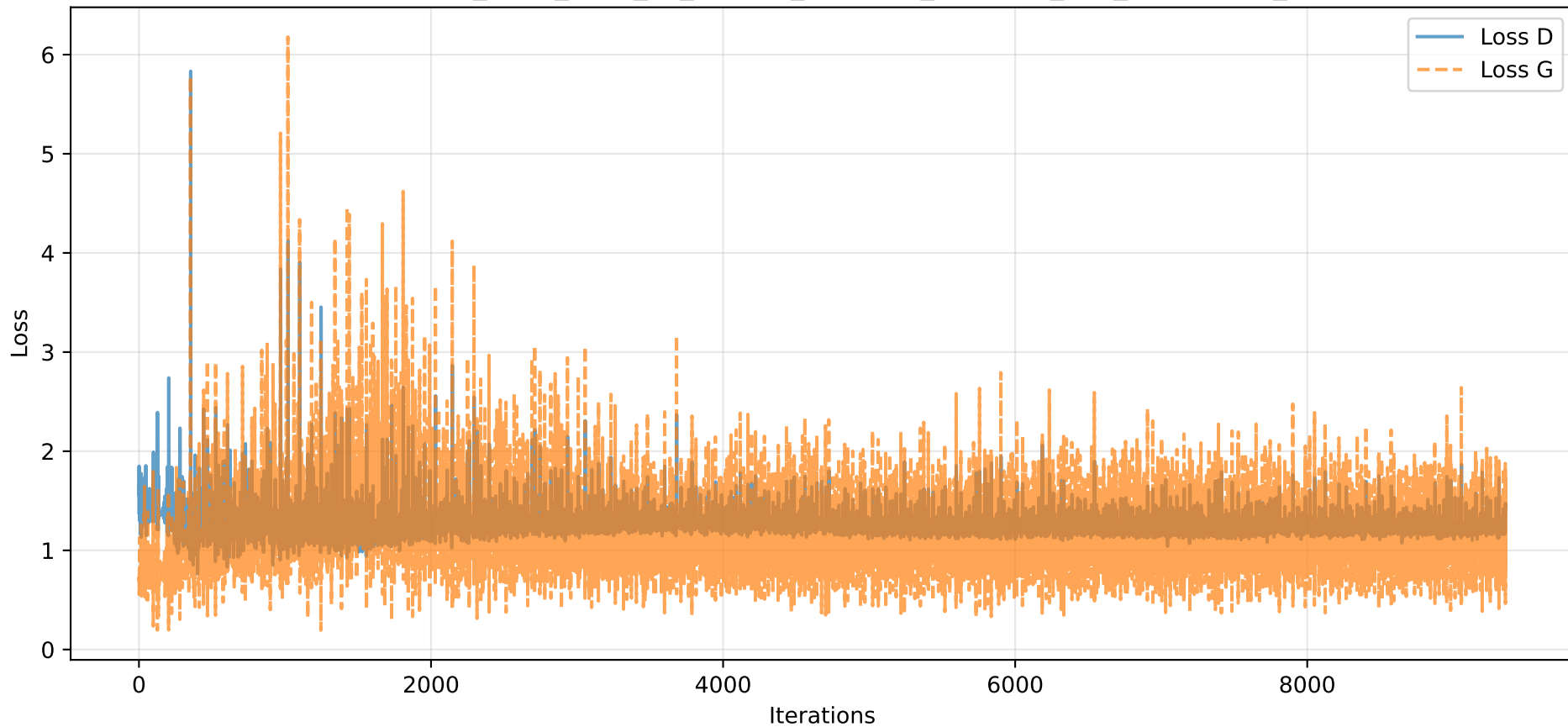
Losses - e20_b128_z100_k1_Oadam_lrG0.002_lrD0.002_l0.9_be0.5-0.99_S42
