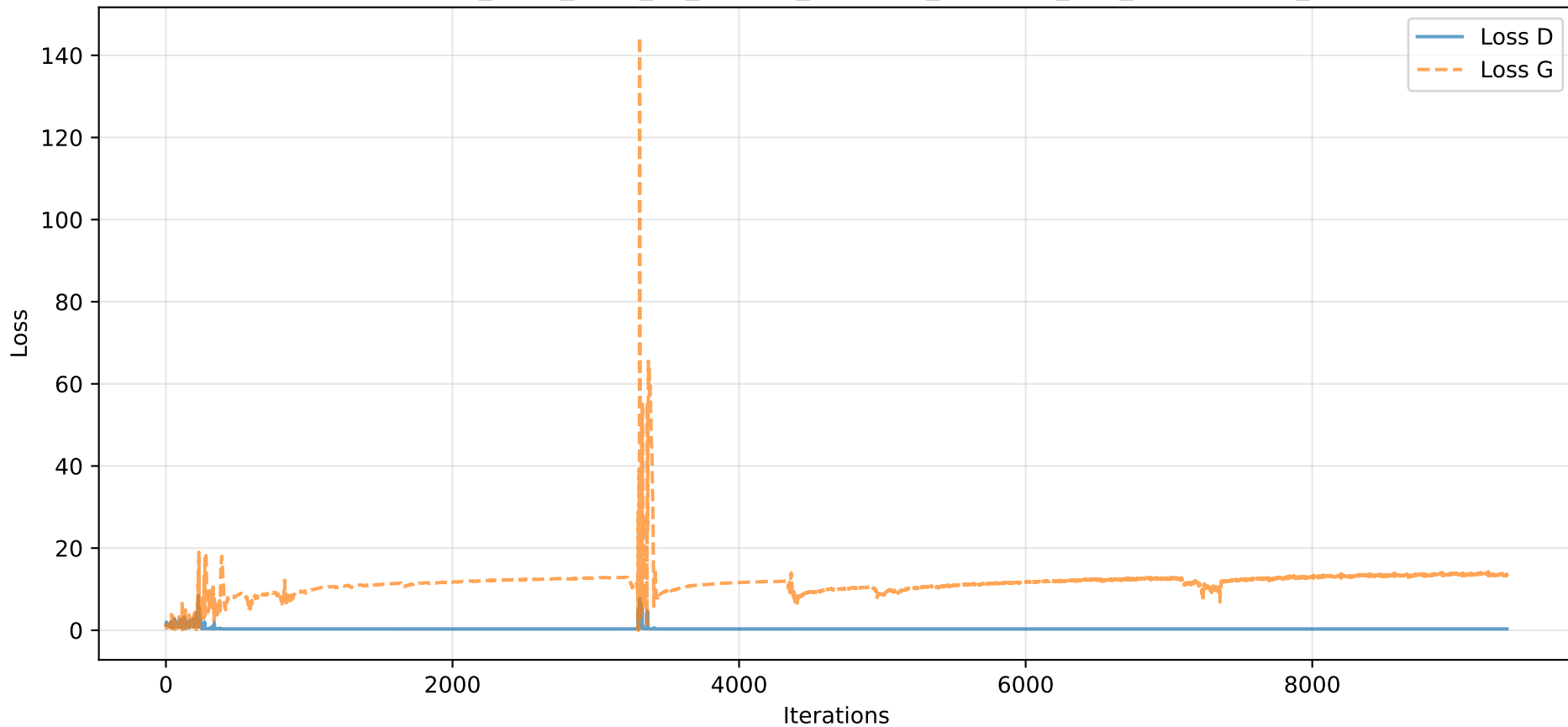
Losses - e20_b128_z100_k1_Oadam_lrG0.002_lrD0.002_l0.9_be0.8-0.999_S42
