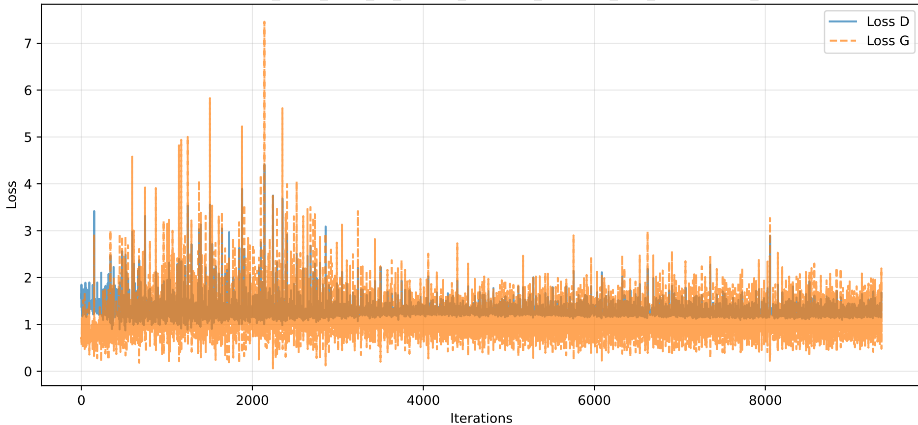
Losses - e20_b128_z100_k1_Oadam_lrG0.002_lrD0.002_l0.9_be0.5-0.999_S42
