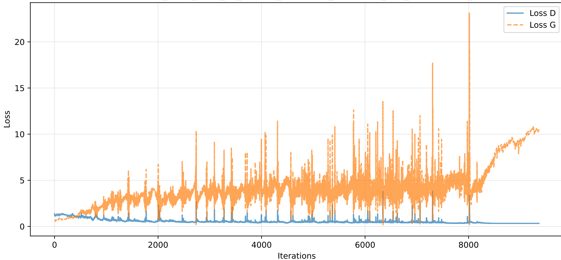
Losses - e20_b128_z100_k1_Oadam_lrG0.0001_lrD0.0001_l0.9_be0.5-0.999_S42
