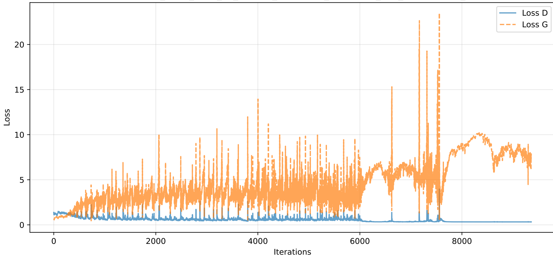
Losses - e20_b128_z100_k1_Oadam_lrG0.0002_lrD0.0002_l0.9_be0.5-0.999_S42
