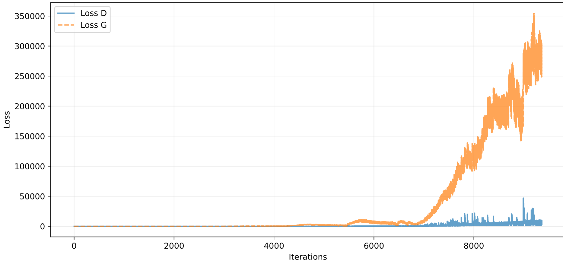
Losses - e20_b128_z100_k1_Olion_lrG0.002_lrD0.002_l0.9_S42
