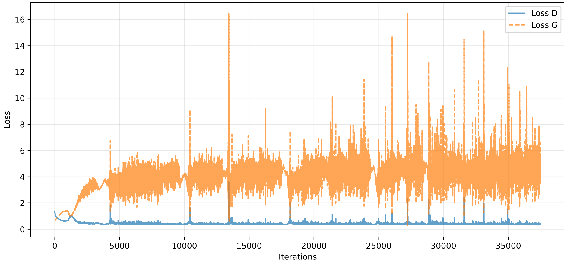
Losses - e20_b32_z100_k1_Osgd_lrG0.002_lrD0.002_l0.9_m0.5_S42
