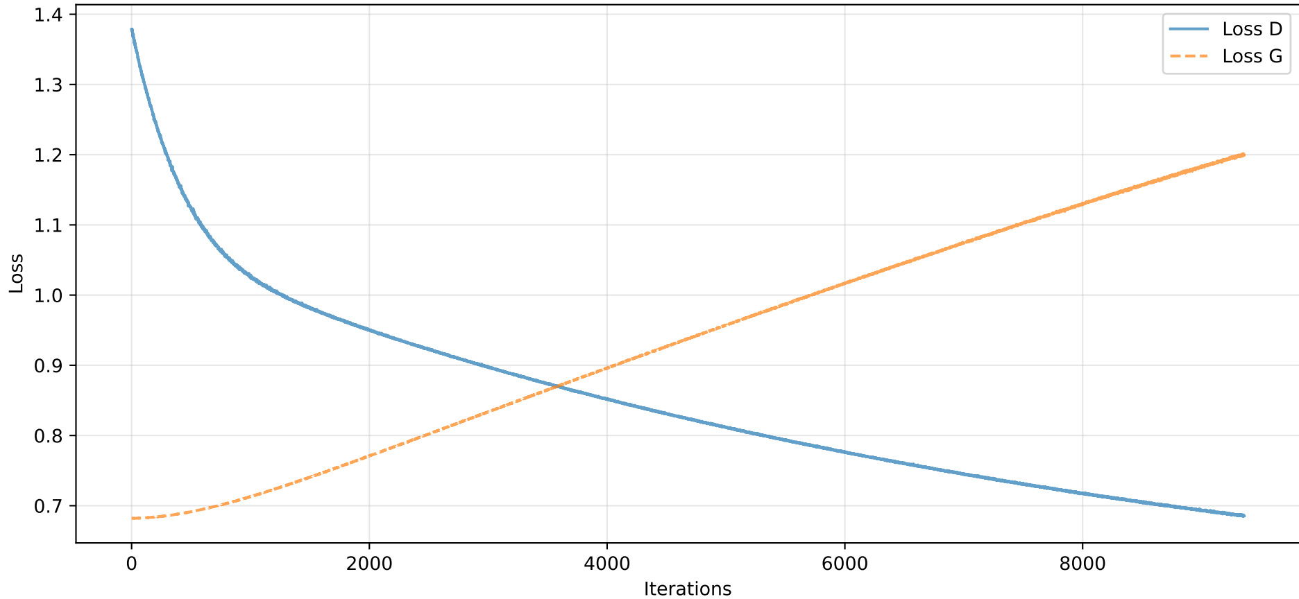
Losses - e20_b128_z100_k1_Osgd_lrG0.0001_lrD0.0001_l0.9_m0.5_S42
