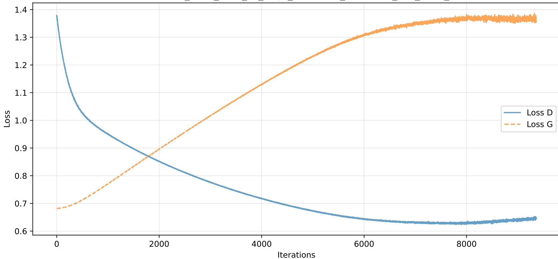
Losses - e20_b128_z100_k1_Osgd_lrG0.0002_lrD0.0002_l0.9_m0.5_S42
