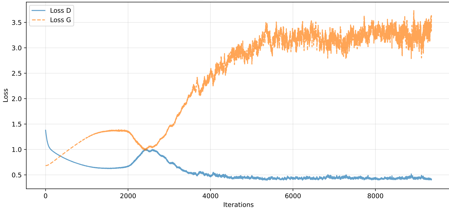
Losses - e20_b128_z100_k1_Osgd_lrG0.001_lrD0.001_l0.9_m0.5_S42
