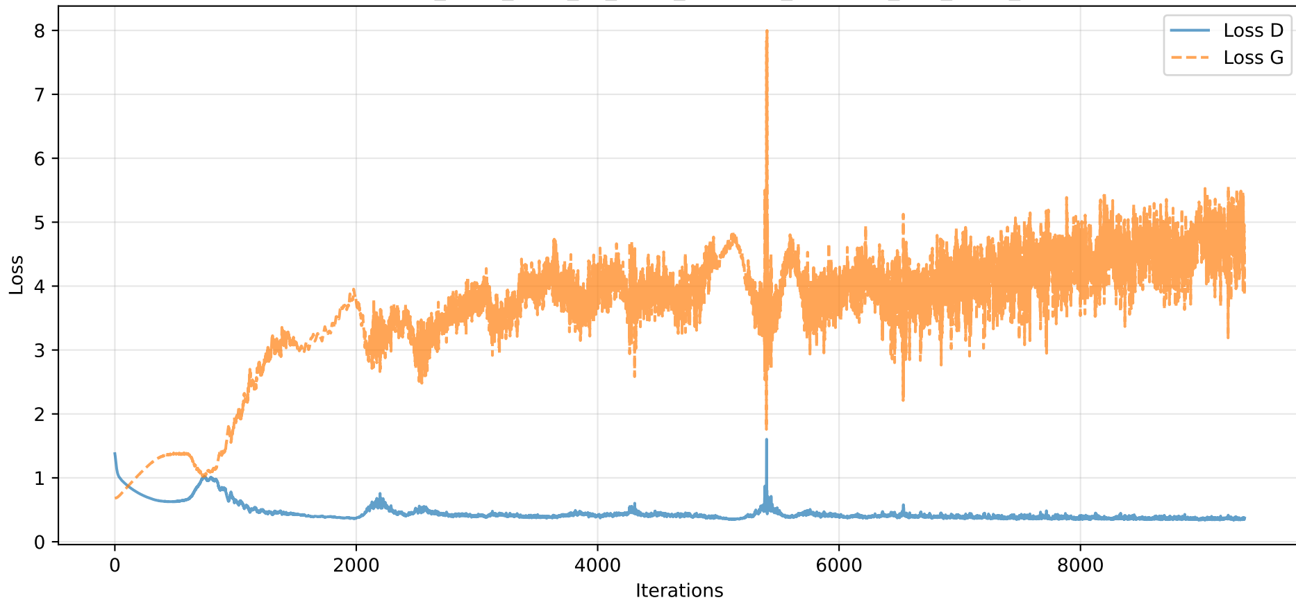
Losses - e20_b128_z100_k1_Osgd_lrG0.002_lrD0.002_l0.9_m0.7_S42
