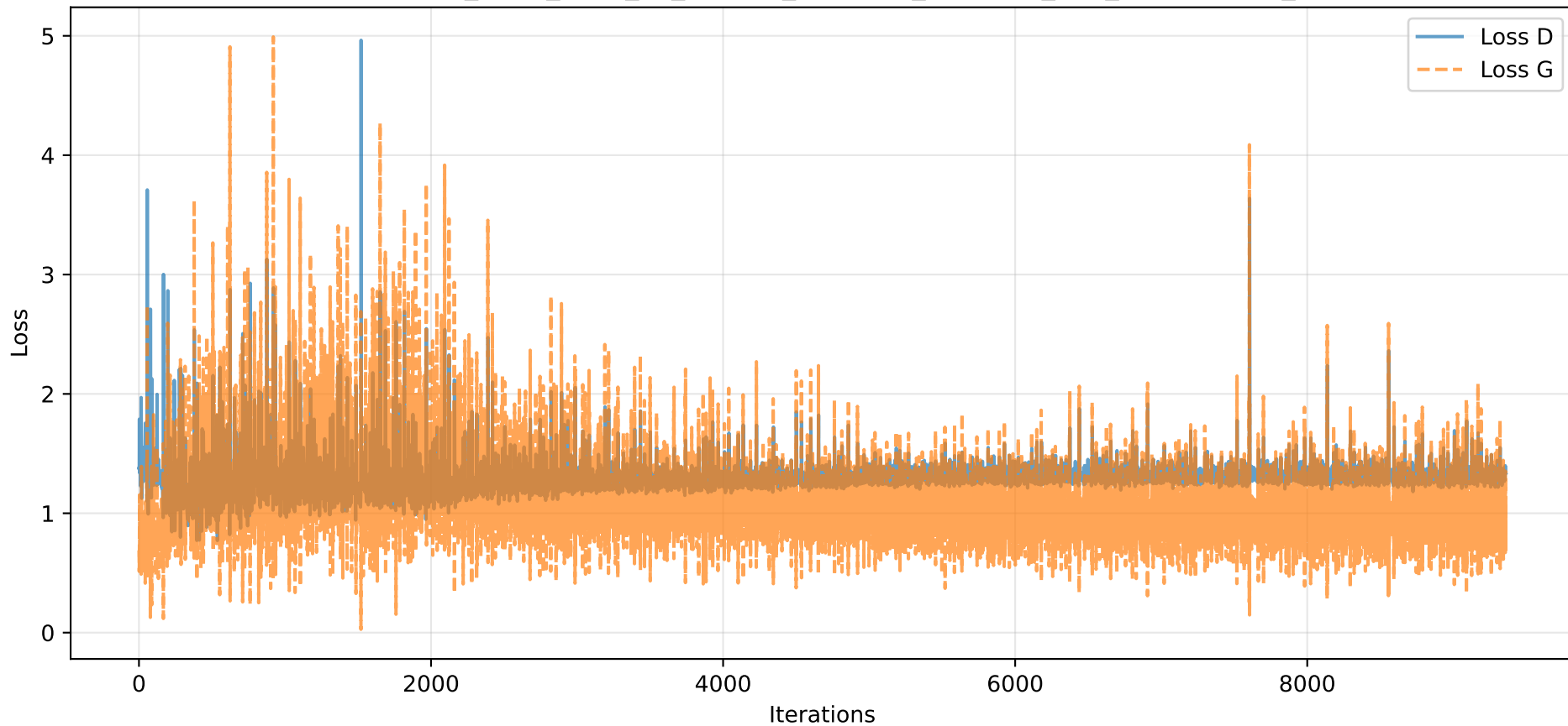
Losses - e20_b128_z100_k1_Oadam_lrG0.001_lrD0.002_l0.9_be0.5-0.999_S42
