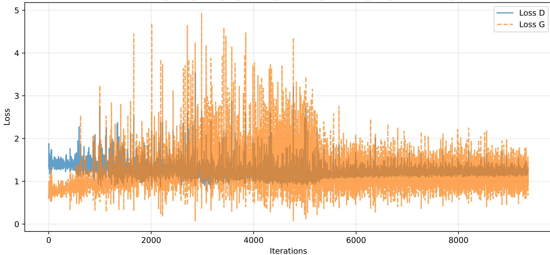
Losses - e20_b128_z100_k1_Oadam_lrG0.002_lrD0.001_l0.9_be0.5-0.999_S42
