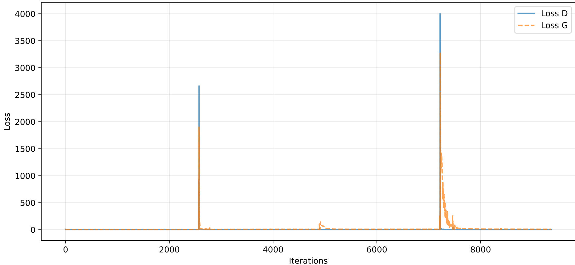
Losses - e20_b128_z100_k1_Oadam_lrG0.002_lrD0.004_l0.9_be0.5-0.999_S42
