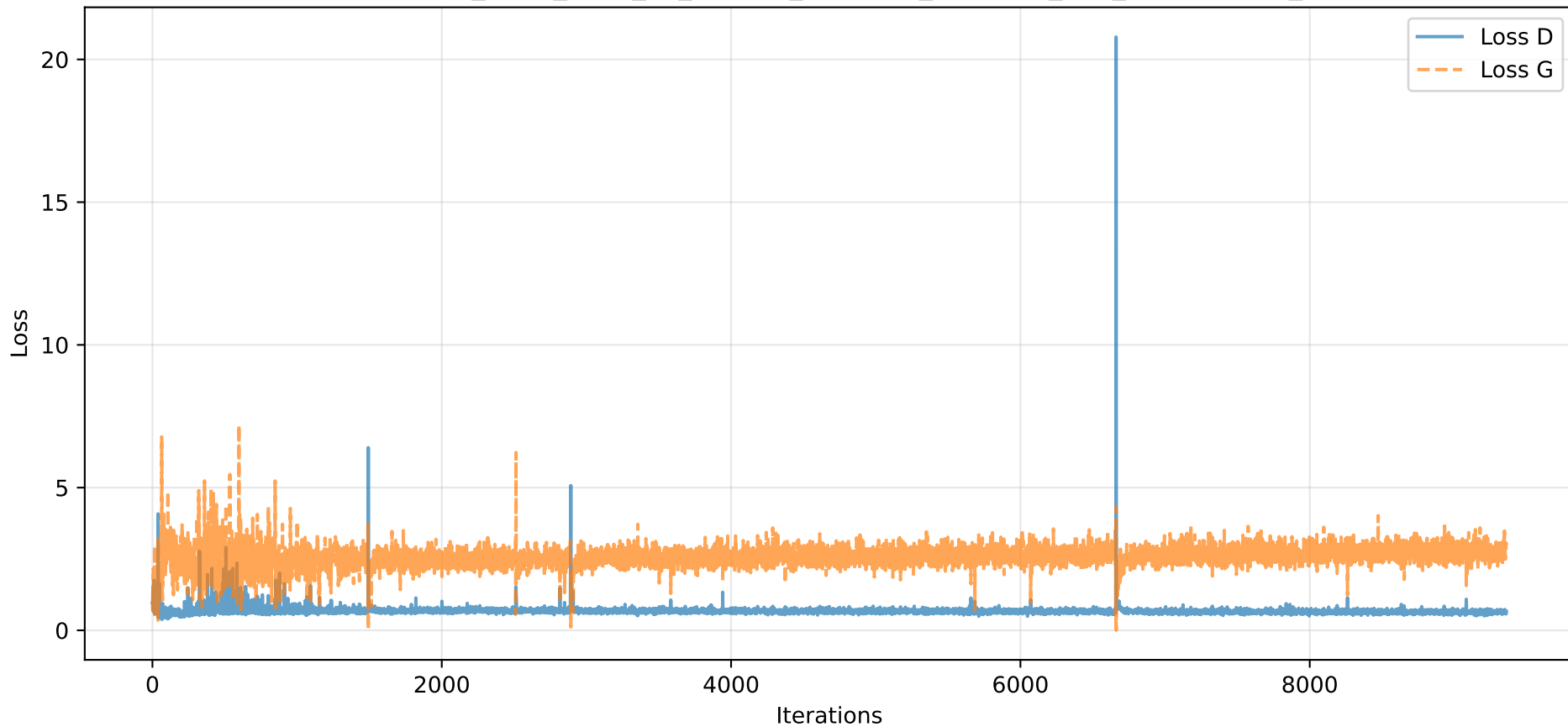
Losses - e20_b128_z100_k5_Oadam_lrG0.002_lrD0.002_l0.9_be0.5-0.999_S42
