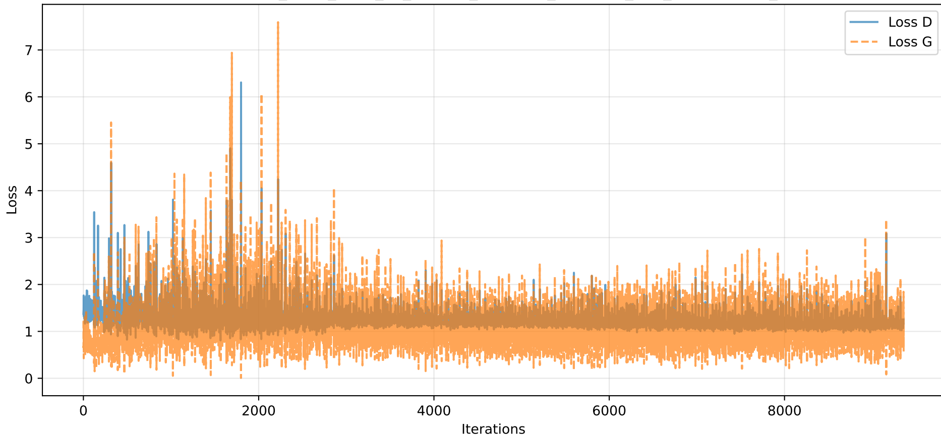
Losses - e20_b128_z100_k1_Oadam_lrG0.002_lrD0.002_l1.0_be0.5-0.999_S42
