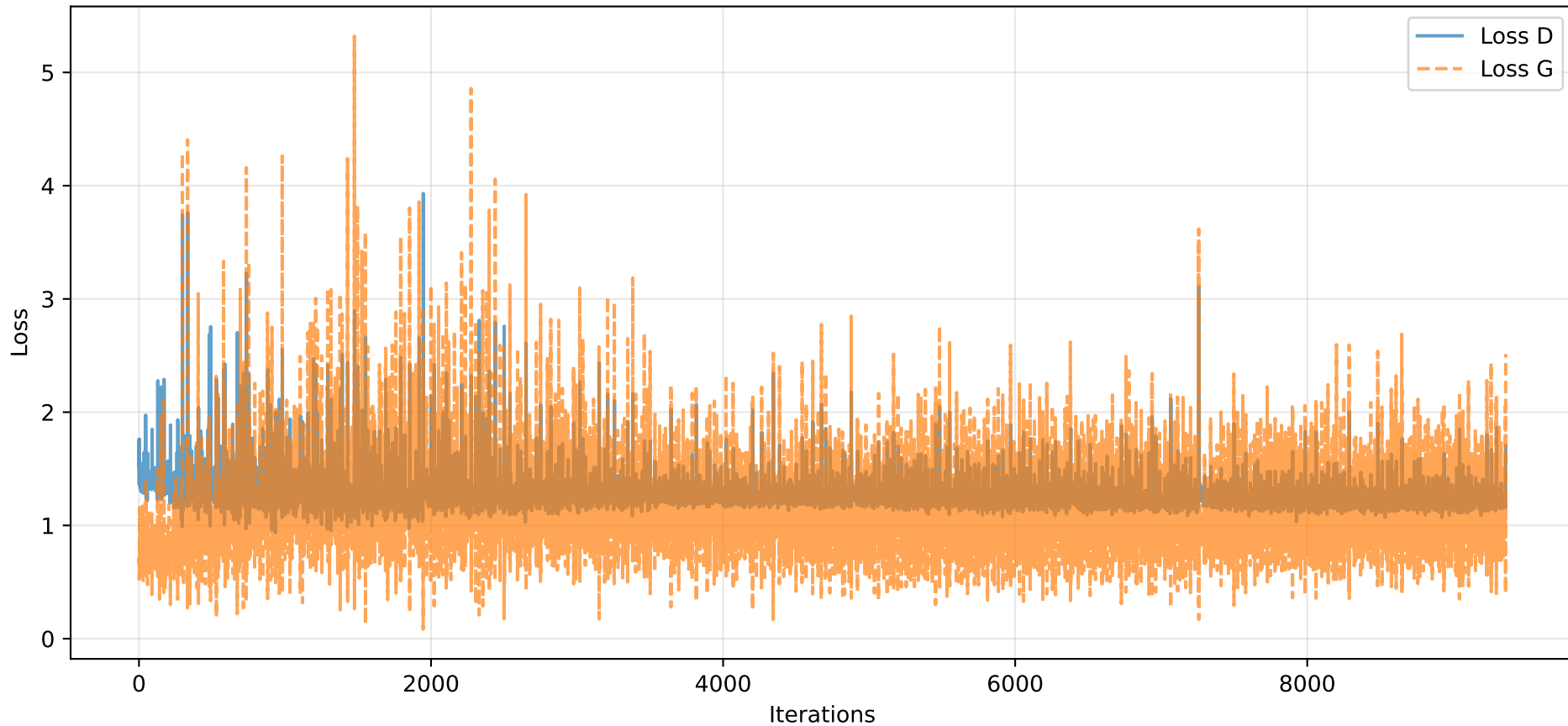
Losses - e20_b128_z150_k1_Oadam_lrG0.002_lrD0.002_l0.9_be0.5-0.999_S42
