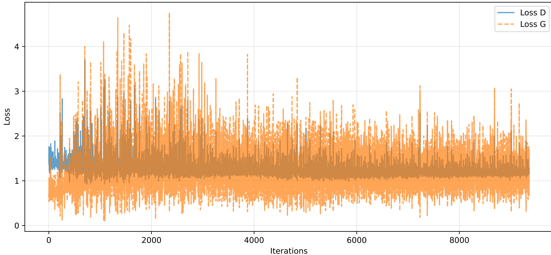
Losses - e20_b128_z200_k1_Oadam_lrG0.002_lrD0.002_l0.9_be0.5-0.999_S42
