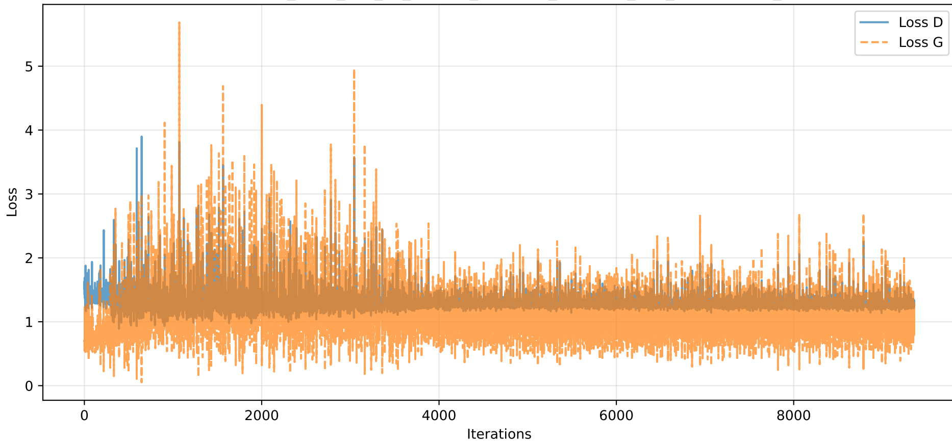
Losses - e20_b128_z50_k1_Oadam_lrG0.002_lrD0.002_l0.9_be0.5-0.999_S42
