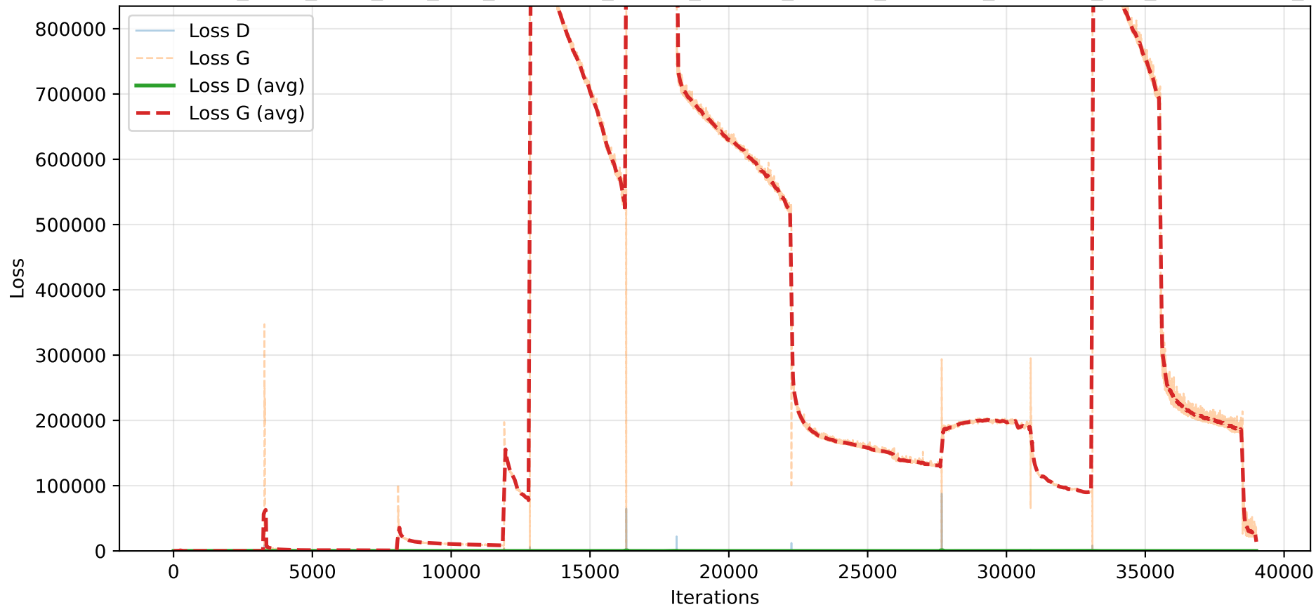
Losses - e100_b128_z100_kD1_kG1_Pbaseline_GArelu_DAlrelu_Oadam_lrG0.002_lrD0.002_l0.9_be0.5-0.999_S42
