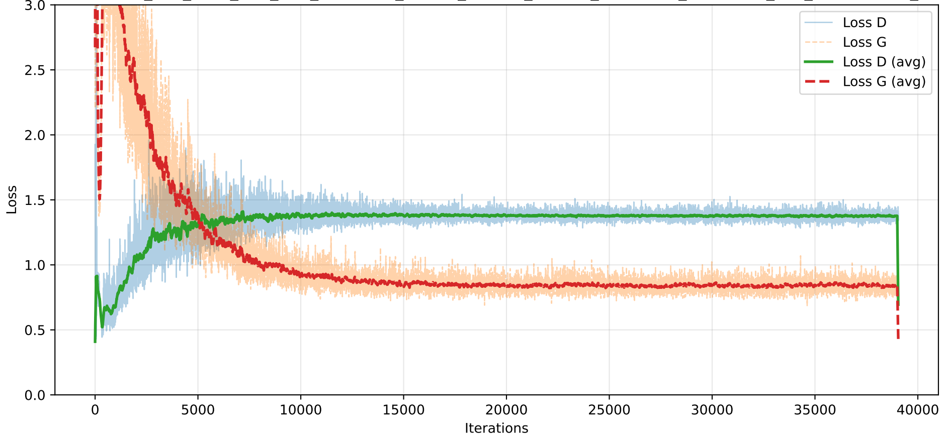
Losses - e50_b64_z100_kD1_kG1_Pbaseline_GArelu_DAlrelu_Oadam_lrG0.0002_lrD0.0002_l0.9_be0.5-0.999_S42
